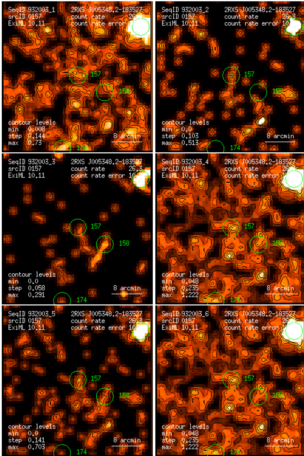
Figure 157: RASS 932003: detection 0157: band rate images, Gaussian filter: (1) PSPC channels 11 – 41, (2) 52 – 90, (3) 91 – 201, (4) 11 – 235, (5) 52 – 201, (6) 11 – 201. Broad band rates in counts/ks. Band rate contour levels in counts/ks/arcmin 2 .
