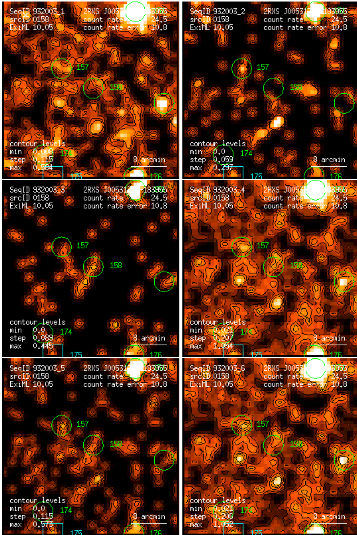
Figure 158: RASS 932003: detection 0158: band rate images, Gaussian filter: (1) PSPC channels 11 – 41, (2) 52 – 90, (3) 91 – 201, (4) 11 – 235, (5) 52 – 201, (6) 11 – 201. Broad band rates in counts/ks. Band rate contour levels in counts/ks/arcmin 2 .
