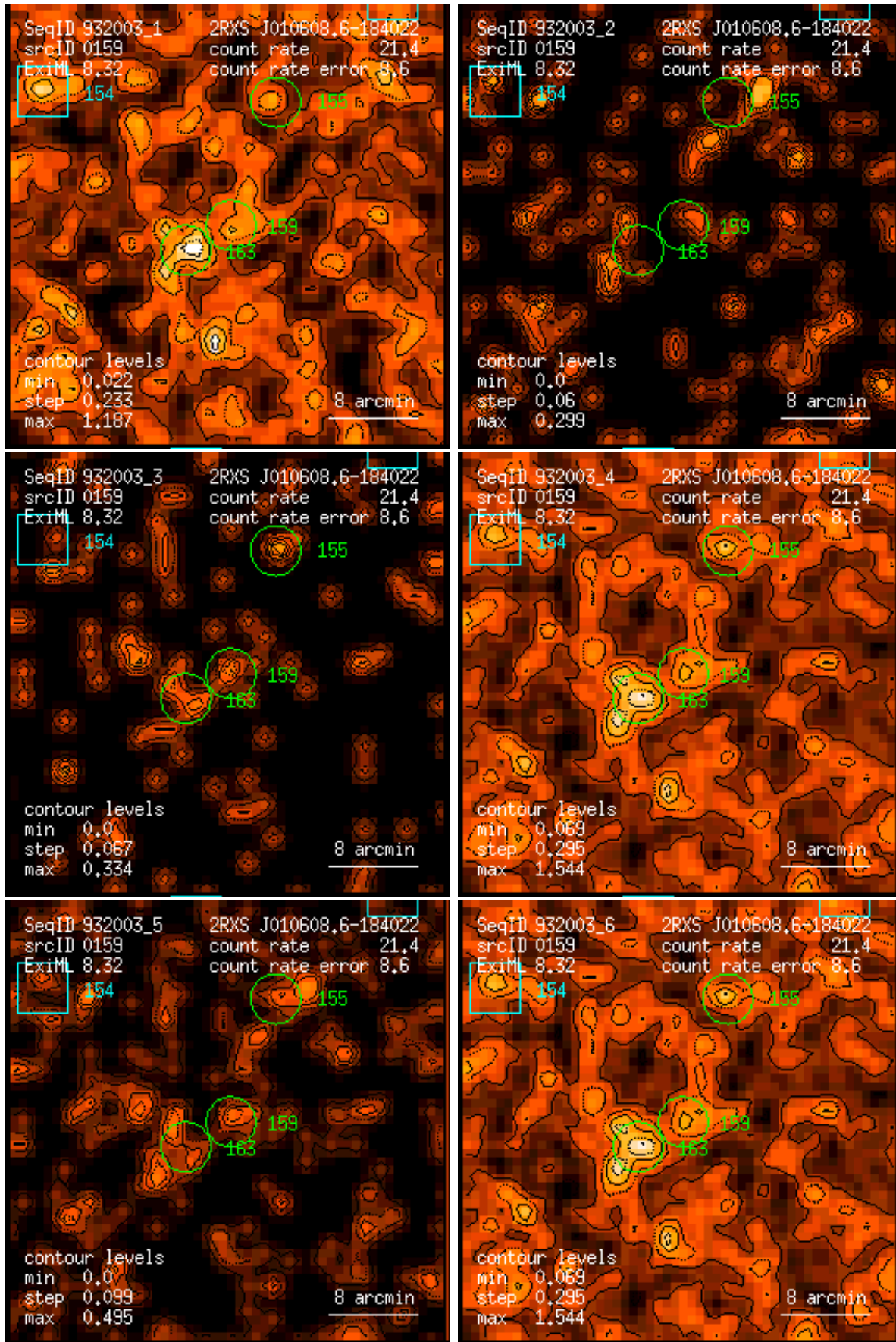
Figure 159: RASS 932003: detection 0159: band rate images, Gaussian filter: (1) PSPC channels 11 – 41, (2) 52 – 90, (3) 91 – 201, (4) 11 – 235, (5) 52 – 201, (6) 11 – 201. Broad band rates in counts/ks. Band rate contour levels in counts/ks/arcmin 2 .
