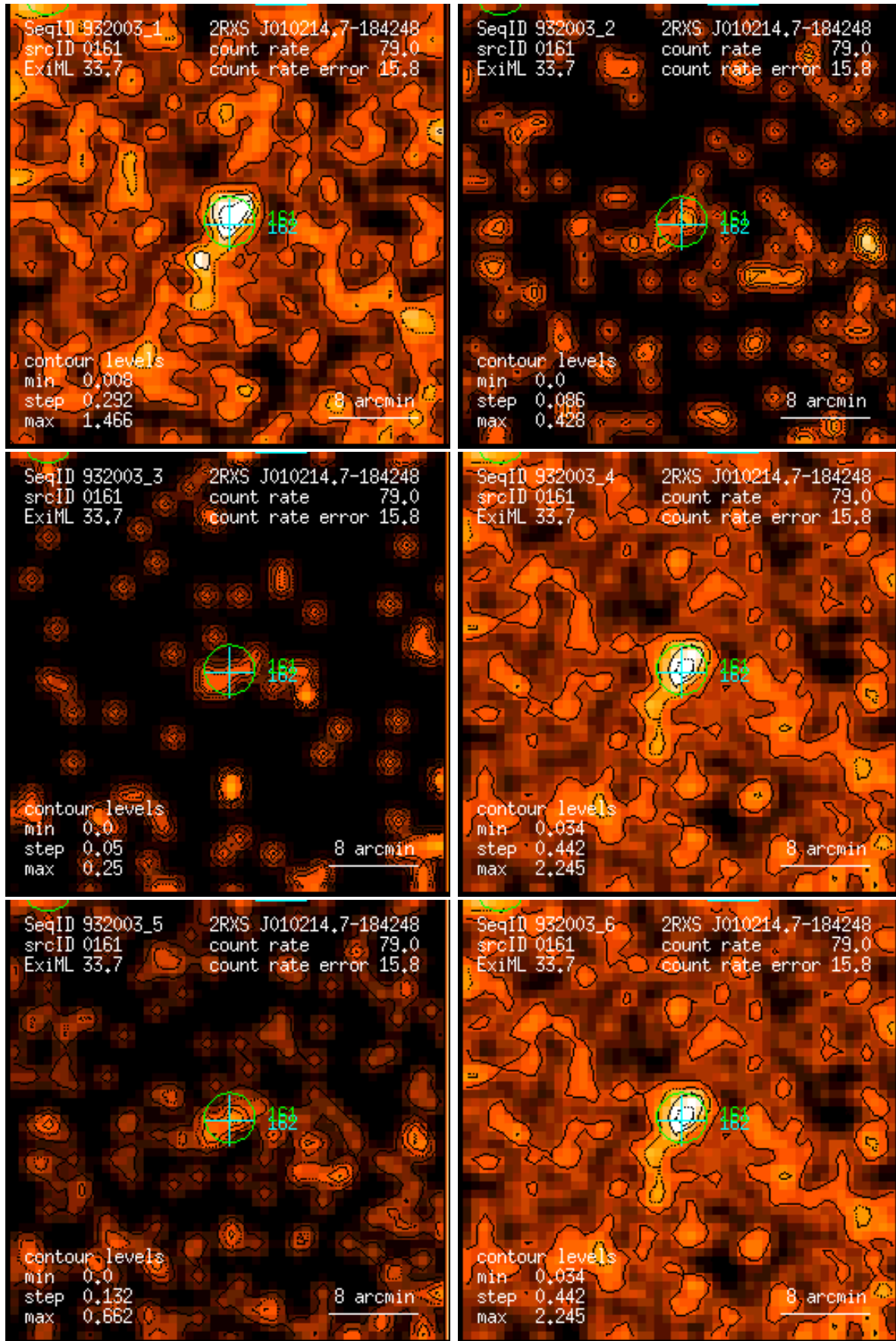
Figure 161: RASS 932003: detection 0161: band rate images, Gaussian filter: (1) PSPC channels 11 – 41, (2) 52 – 90, (3) 91 – 201, (4) 11 – 235, (5) 52 – 201, (6) 11 – 201. Broad band rates in counts/ks. Band rate contour levels in counts/ks/arcmin 2 .
