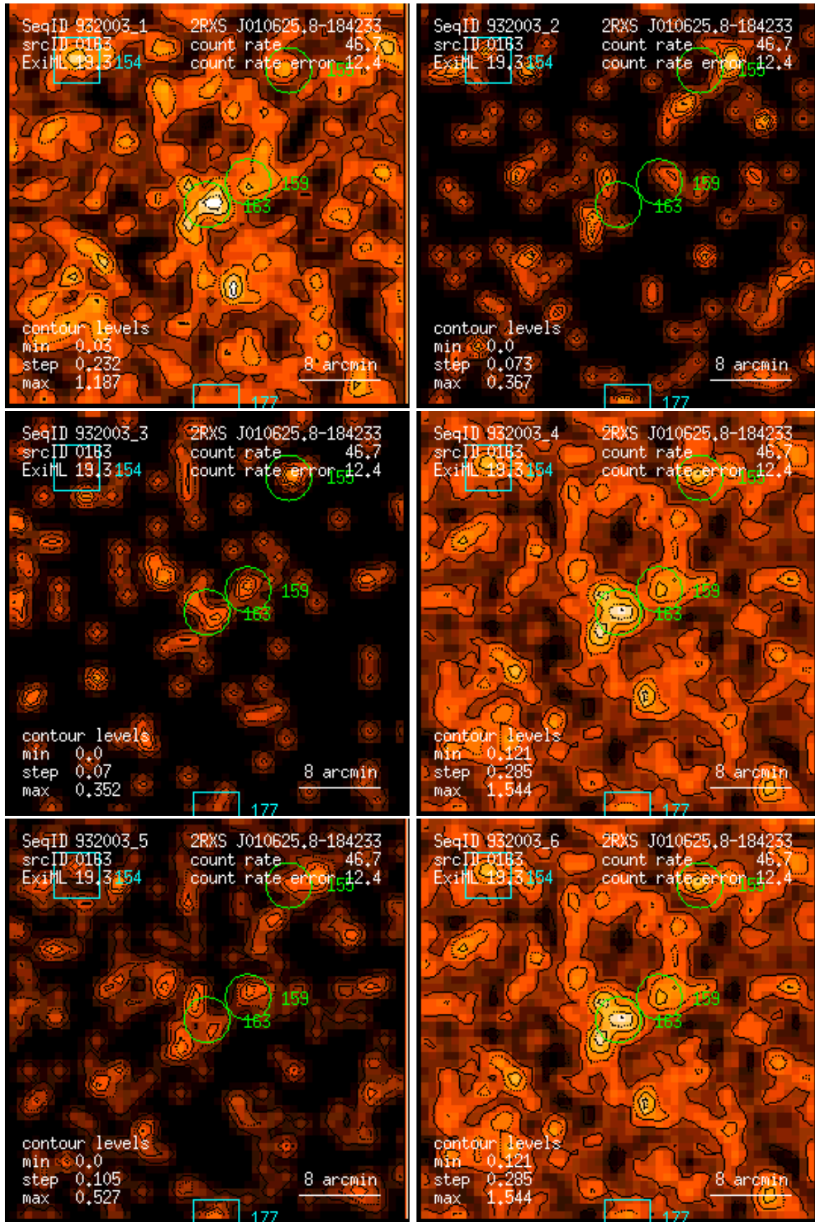
Figure 163: RASS 932003: detection 0163: band rate images, Gaussian filter: (1) PSPC channels 11 – 41, (2) 52 – 90, (3) 91 – 201, (4) 11 – 235, (5) 52 – 201, (6) 11 – 201. Broad band rates in counts/ks. Band rate contour levels in counts/ks/arcmin 2 .
