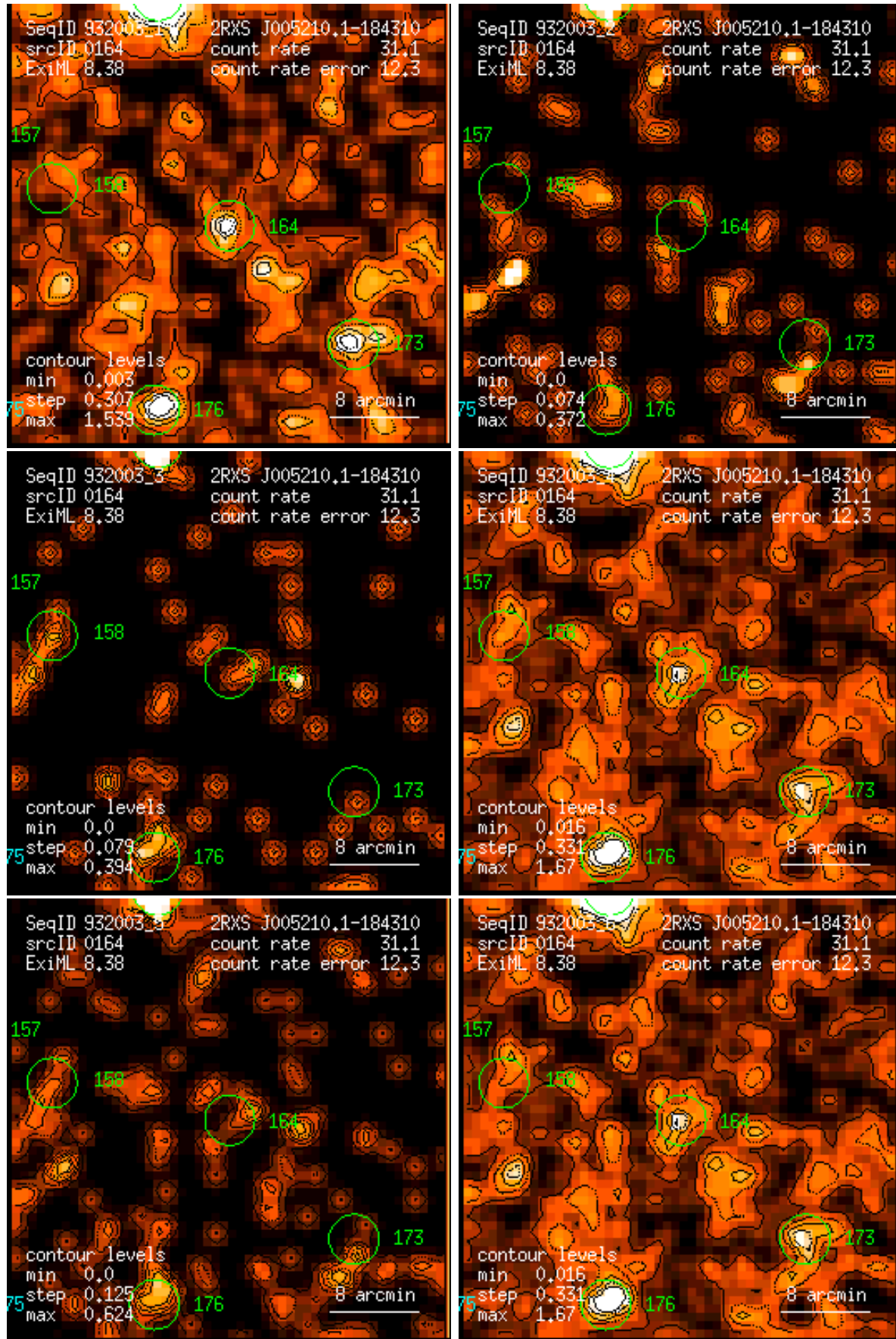
Figure 164: RASS 932003: detection 0164: band rate images, Gaussian filter: (1) PSPC channels 11 – 41, (2) 52 – 90, (3) 91 – 201, (4) 11 – 235, (5) 52 – 201, (6) 11 – 201. Broad band rates in counts/ks. Band rate contour levels in counts/ks/arcmin 2 .
