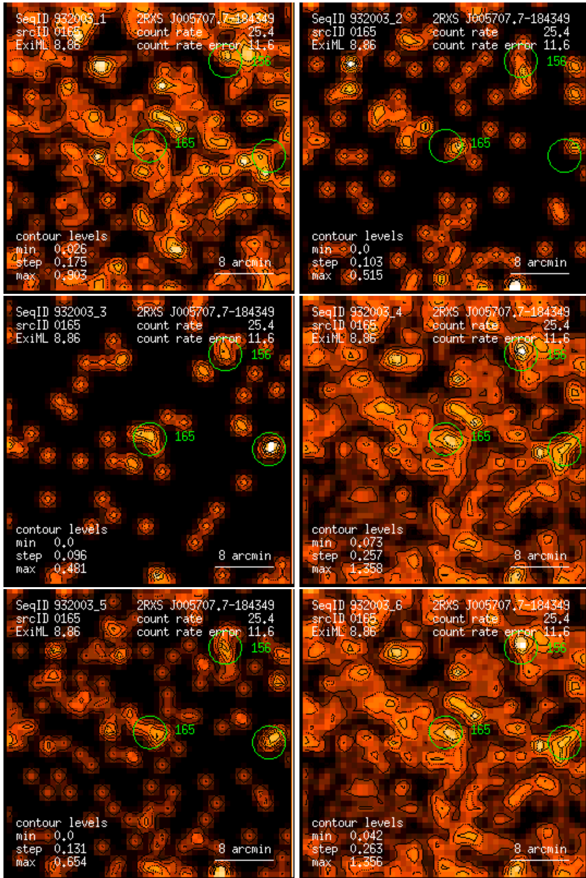
Figure 165: RASS 932003: detection 0165: band rate images, Gaussian filter: (1) PSPC channels 11 – 41, (2) 52 – 90, (3) 91 – 201, (4) 11 – 235, (5) 52 – 201, (6) 11 – 201. Broad band rates in counts/ks. Band rate contour levels in counts/ks/arcmin 2 .
