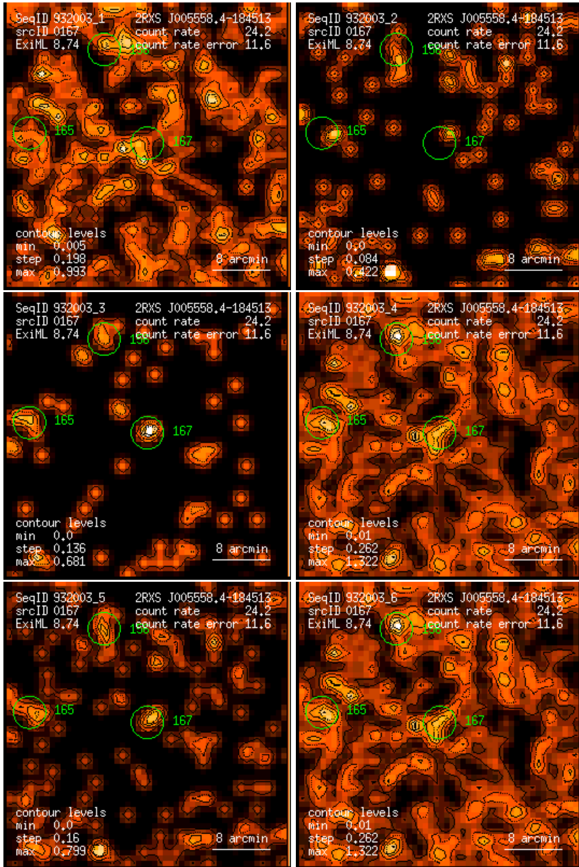
Figure 167: RASS 932003: detection 0167: band rate images, Gaussian filter: (1) PSPC channels 11 – 41, (2) 52 – 90, (3) 91 – 201, (4) 11 – 235, (5) 52 – 201, (6) 11 – 201. Broad band rates in counts/ks. Band rate contour levels in counts/ks/arcmin 2 .
