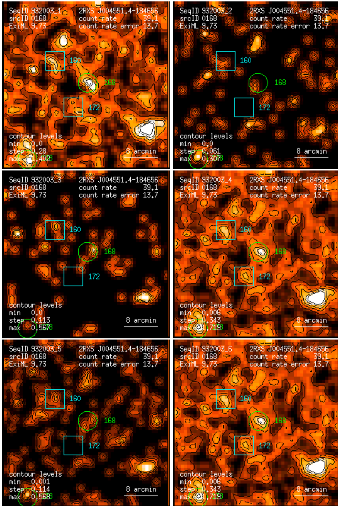
Figure 168: RASS 932003: detection 0168: band rate images, Gaussian filter: (1) PSPC channels 11 – 41, (2) 52 – 90, (3) 91 – 201, (4) 11 – 235, (5) 52 – 201, (6) 11 – 201. Broad band rates in counts/ks. Band rate contour levels in counts/ks/arcmin 2 .
