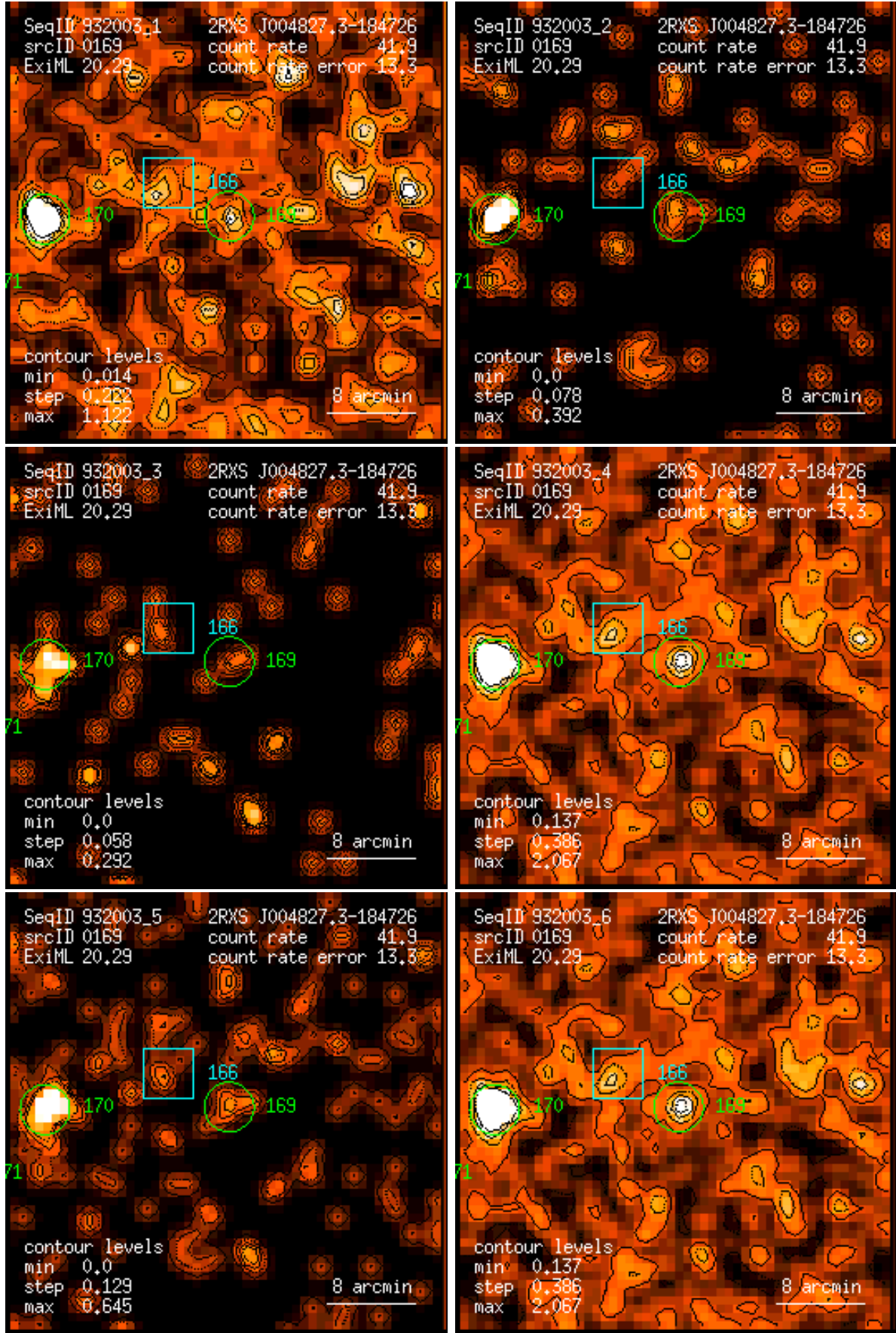
Figure 169: RASS 932003: detection 0169: band rate images, Gaussian filter: (1) PSPC channels 11 – 41, (2) 52 – 90, (3) 91 – 201, (4) 11 – 235, (5) 52 – 201, (6) 11 – 201. Broad band rates in counts/ks. Band rate contour levels in counts/ks/arcmin 2 .
