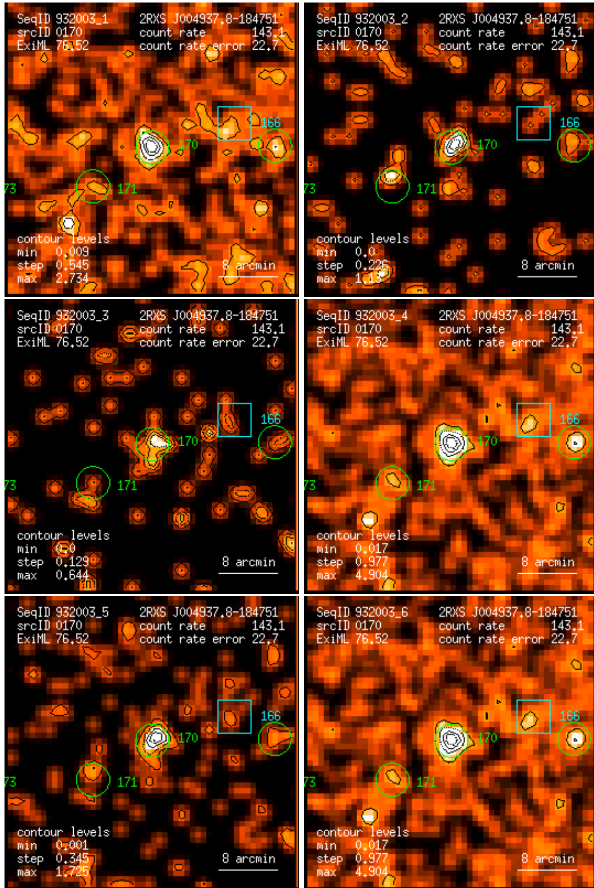
Figure 170: RASS 932003: detection 0170: band rate images, Gaussian filter: (1) PSPC channels 11 – 41, (2) 52 – 90, (3) 91 – 201, (4) 11 – 235, (5) 52 – 201, (6) 11 – 201. Broad band rates in counts/ks. Band rate contour levels in counts/ks/arcmin 2 .
