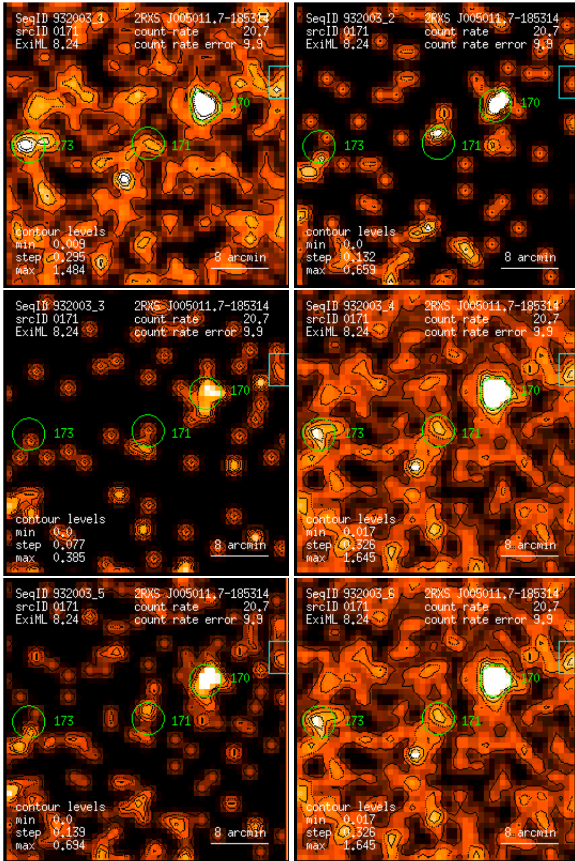
Figure 171: RASS 932003: detection 0171: band rate images, Gaussian filter: (1) PSPC channels 11 – 41, (2) 52 – 90, (3) 91 – 201, (4) 11 – 235, (5) 52 – 201, (6) 11 – 201. Broad band rates in counts/ks. Band rate contour levels in counts/ks/arcmin 2 .
