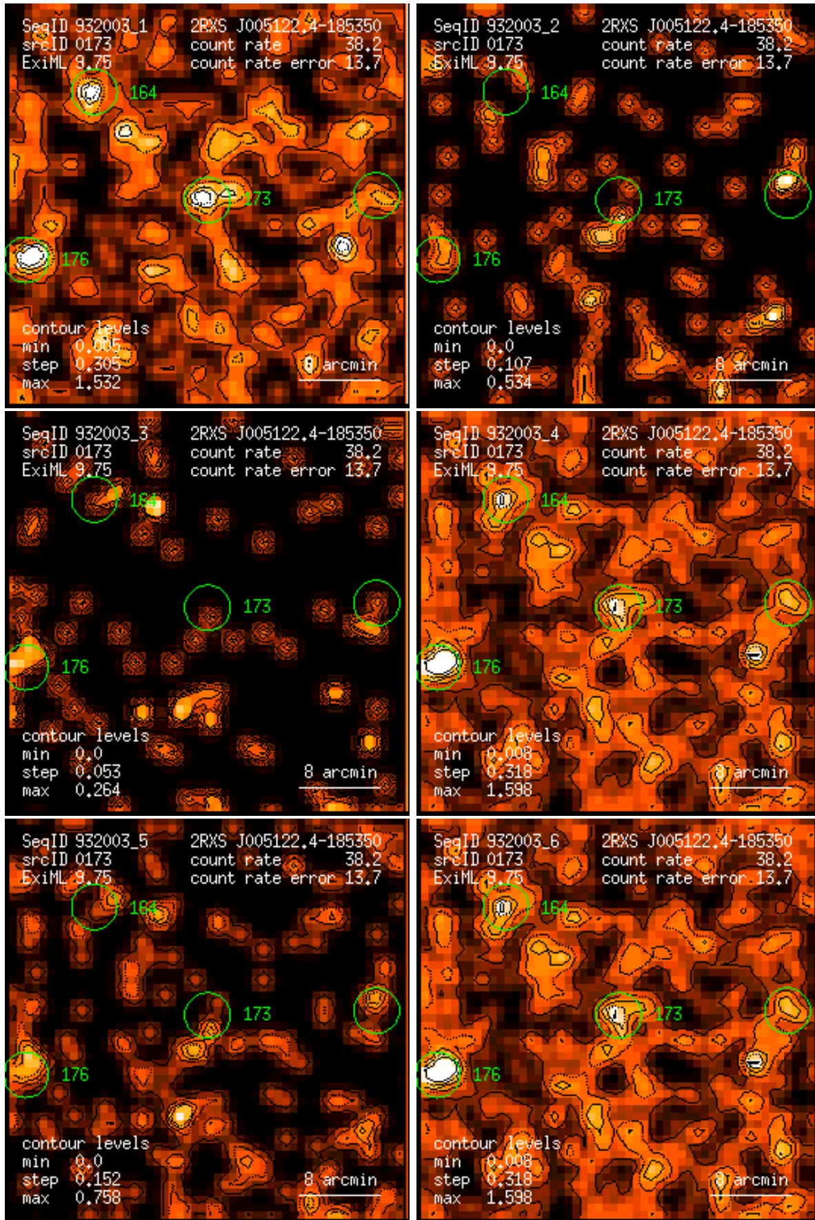
Figure 173: RASS 932003: detection 0173: band rate images, Gaussian filter: (1) PSPC channels 11 – 41, (2) 52 – 90, (3) 91 – 201, (4) 11 – 235, (5) 52 – 201, (6) 11 – 201. Broad band rates in counts/ks. Band rate contour levels in counts/ks/arcmin 2 .
