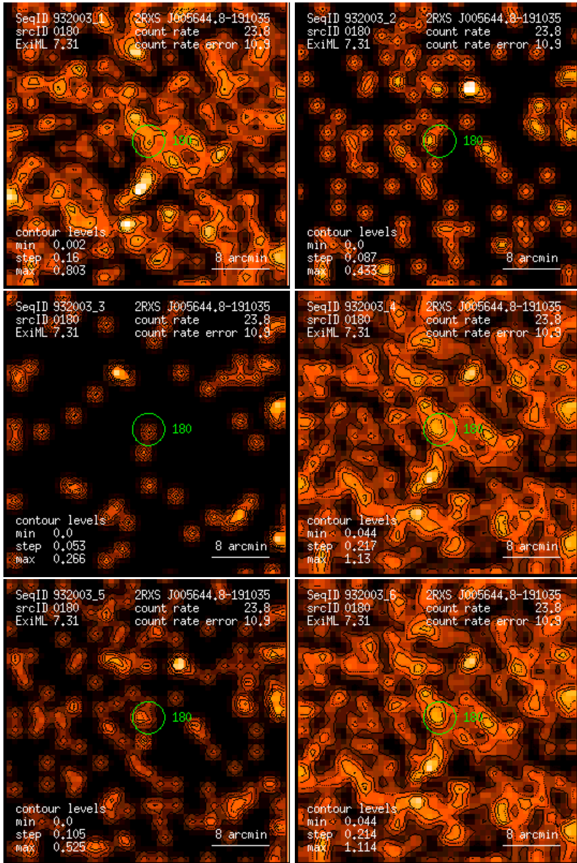
Figure 180: RASS 932003: detection 0180: band rate images, Gaussian filter: (1) PSPC channels 11 – 41, (2) 52 – 90, (3) 91 – 201, (4) 11 – 235, (5) 52 – 201, (6) 11 – 201. Broad band rates in counts/ks. Band rate contour levels in counts/ks/arcmin 2 .
