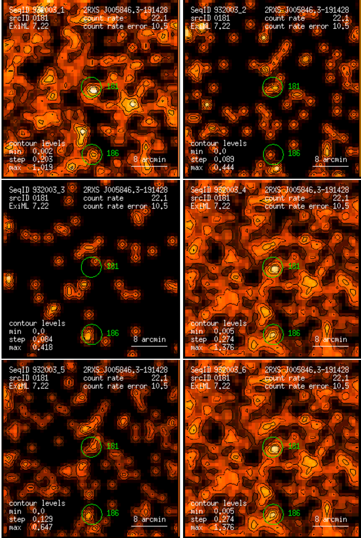
Figure 181: RASS 932003: detection 0181: band rate images, Gaussian filter: (1) PSPC channels 11 – 41, (2) 52 – 90, (3) 91 – 201, (4) 11 – 235, (5) 52 – 201, (6) 11 – 201. Broad band rates in counts/ks. Band rate contour levels in counts/ks/arcmin 2 .
