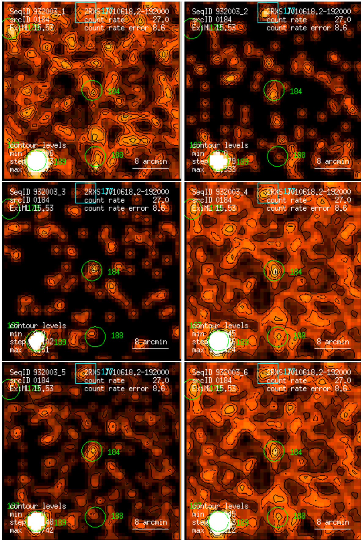
Figure 184: RASS 932003: detection 0184: band rate images, Gaussian filter: (1) PSPC channels 11 – 41, (2) 52 – 90, (3) 91 – 201, (4) 11 – 235, (5) 52 – 201, (6) 11 – 201. Broad band rates in counts/ks. Band rate contour levels in counts/ks/arcmin 2 .
