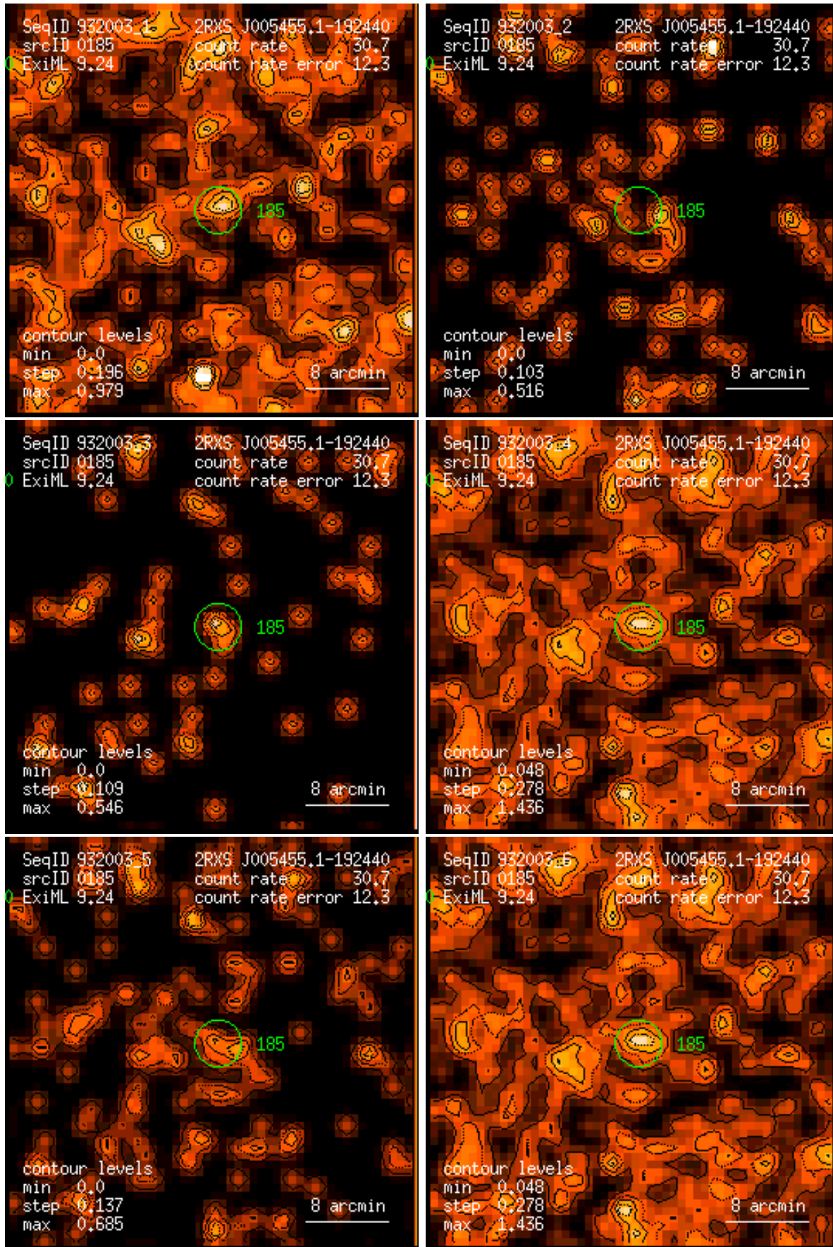
Figure 185: RASS 932003: detection 0185: band rate images, Gaussian filter: (1) PSPC channels 11 – 41, (2) 52 – 90, (3) 91 – 201, (4) 11 – 235, (5) 52 – 201, (6) 11 – 201. Broad band rates in counts/ks. Band rate contour levels in counts/ks/arcmin 2 .
