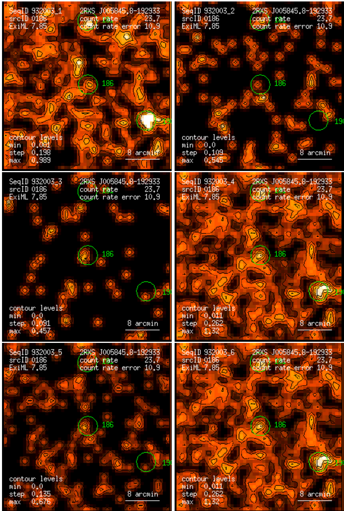
Figure 186: RASS 932003: detection 0186: band rate images, Gaussian filter: (1) PSPC channels 11 – 41, (2) 52 – 90, (3) 91 – 201, (4) 11 – 235, (5) 52 – 201, (6) 11 – 201. Broad band rates in counts/ks. Band rate contour levels in counts/ks/arcmin 2 .
