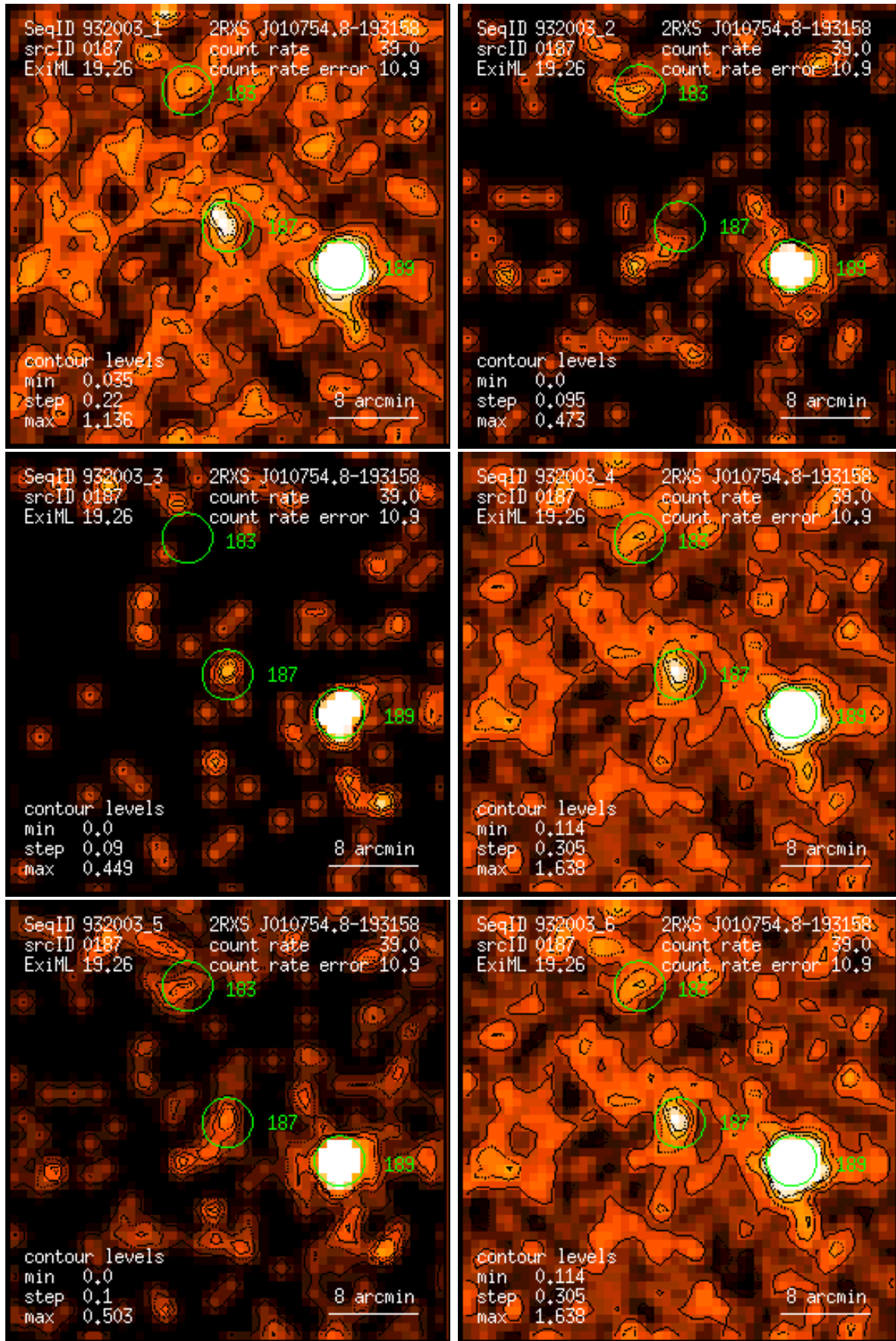
Figure 187: RASS 932003: detection 0187: band rate images, Gaussian filter: (1) PSPC channels 11 – 41, (2) 52 – 90, (3) 91 – 201, (4) 11 – 235, (5) 52 – 201, (6) 11 – 201. Broad band rates in counts/ks. Band rate contour levels in counts/ks/arcmin 2 .
