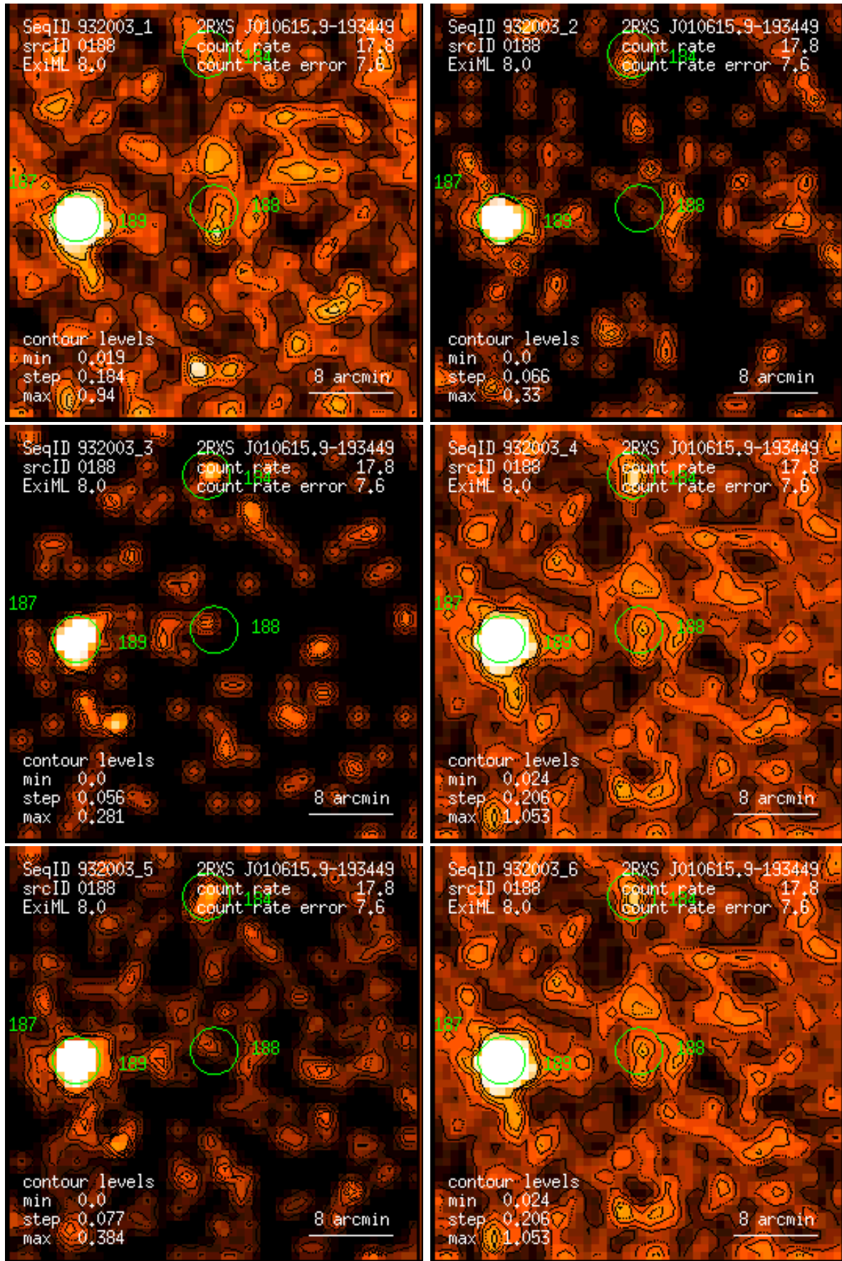
Figure 188: RASS 932003: detection 0188: band rate images, Gaussian filter: (1) PSPC channels 11 – 41, (2) 52 – 90, (3) 91 – 201, (4) 11 – 235, (5) 52 – 201, (6) 11 – 201. Broad band rates in counts/ks. Band rate contour levels in counts/ks/arcmin 2 .
