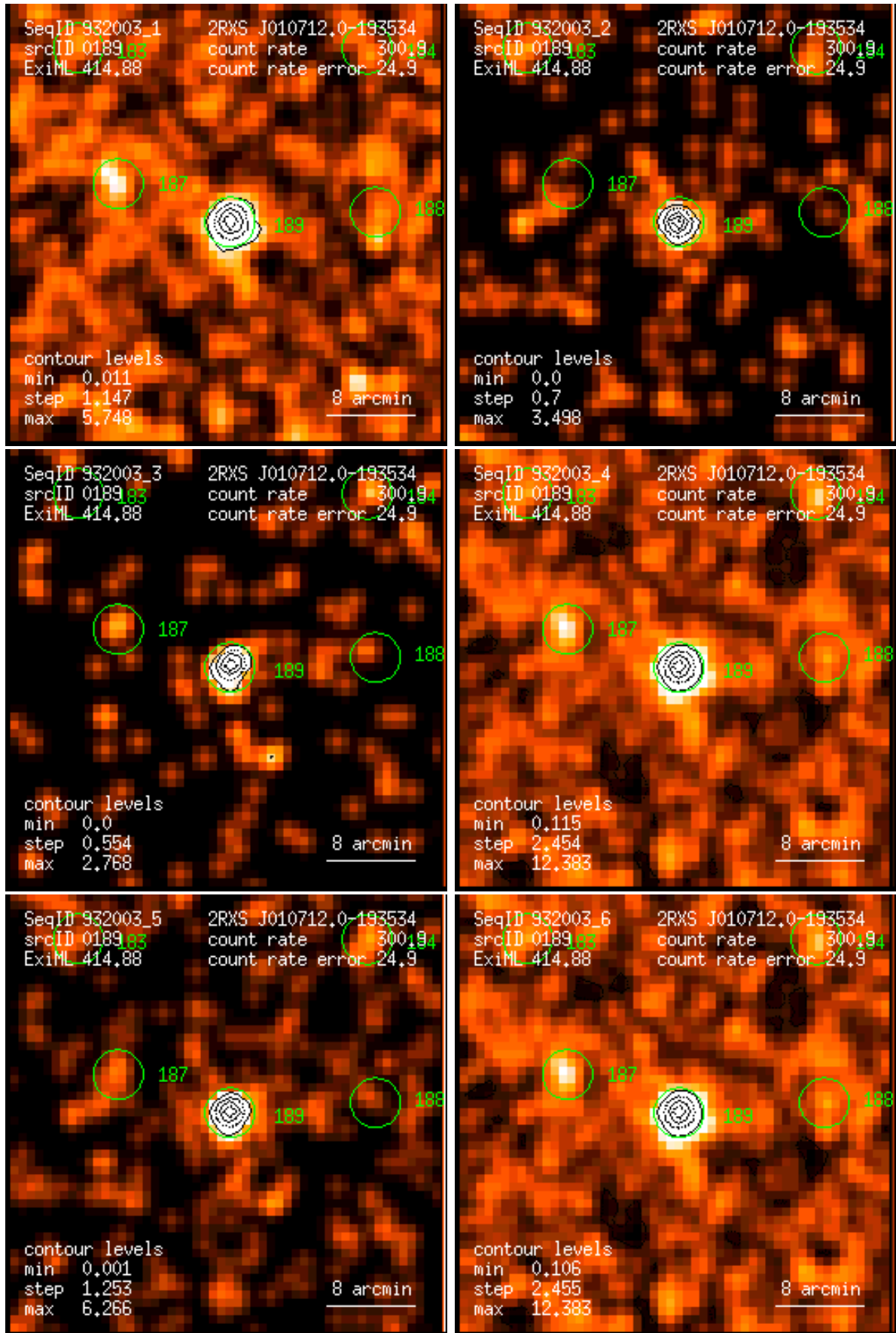
Figure 189: RASS 932003: detection 0189: band rate images, Gaussian filter: (1) PSPC channels 11 – 41, (2) 52 – 90, (3) 91 – 201, (4) 11 – 235, (5) 52 – 201, (6) 11 – 201. Broad band rates in counts/ks. Band rate contour levels in counts/ks/arcmin 2 .
