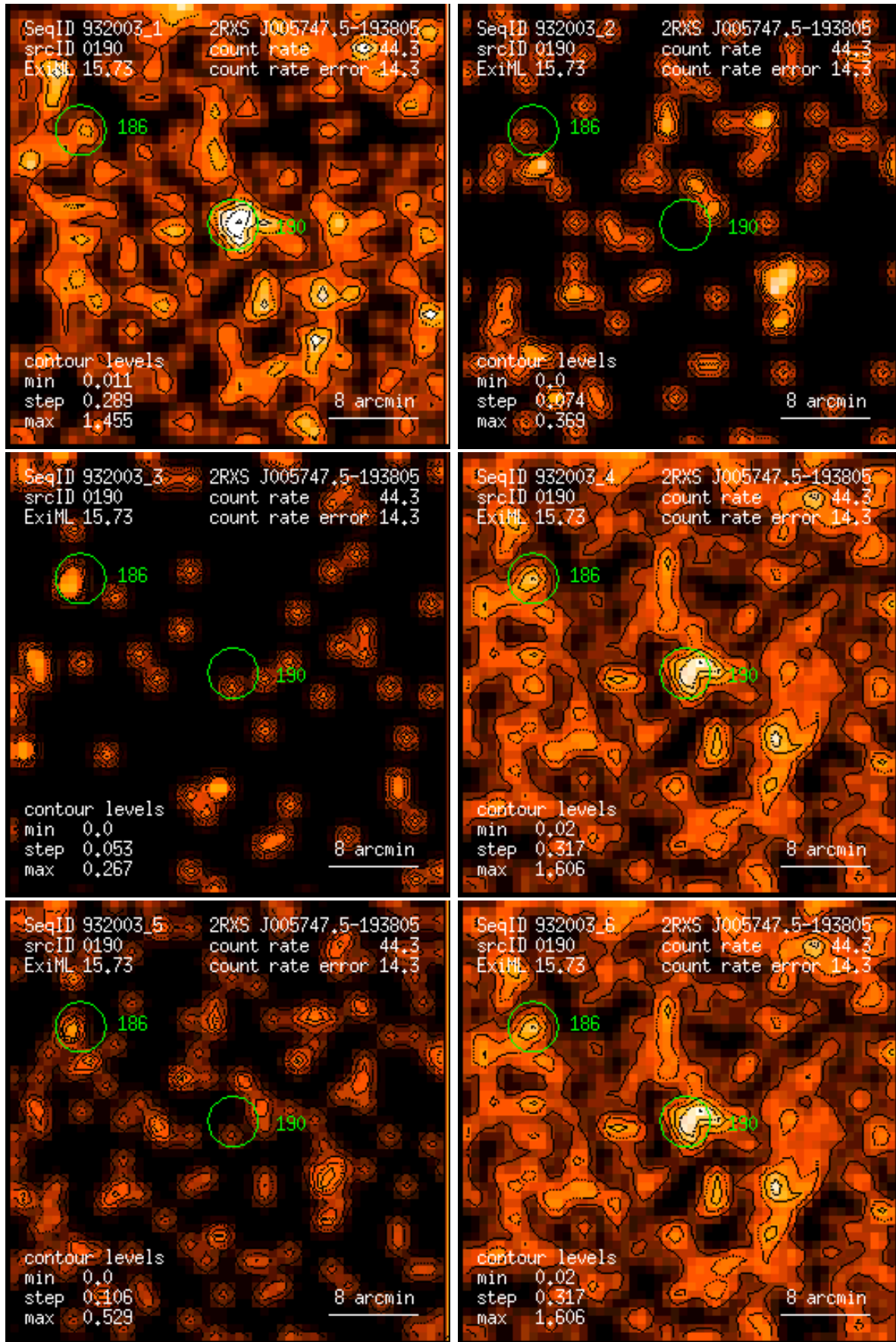
Figure 190: RASS 932003: detection 0190: band rate images, Gaussian filter: (1) PSPC channels 11 – 41, (2) 52 – 90, (3) 91 – 201, (4) 11 – 235, (5) 52 – 201, (6) 11 – 201. Broad band rates in counts/ks. Band rate contour levels in counts/ks/arcmin 2 .
