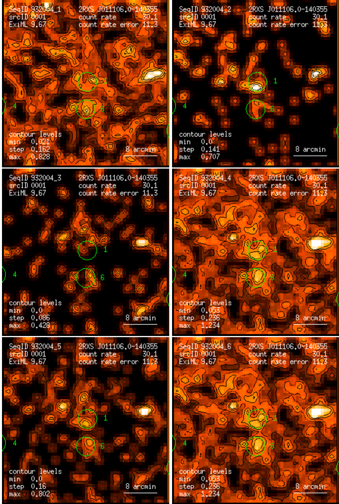
Figure 1: RASS 932004: detection 0001: band rate images, Gaussian filter: (1) PSPC channels 11 – 41, (2) 52 – 90, (3) 91 – 201, (4) 11 – 235, (5) 52 – 201, (6) 11 – 201. Broad band rates in counts/ks. Band rate contour levels in counts/ks/arcmin 2 .
