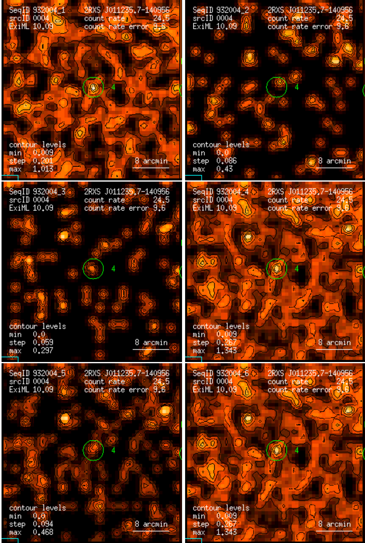
Figure 4: RASS 932004: detection 0004: band rate images, Gaussian filter: (1) PSPC channels 11 – 41, (2) 52 – 90, (3) 91 – 201, (4) 11 – 235, (5) 52 – 201, (6) 11 – 201. Broad band rates in counts/ks. Band rate contour levels in counts/ks/arcmin 2 .
