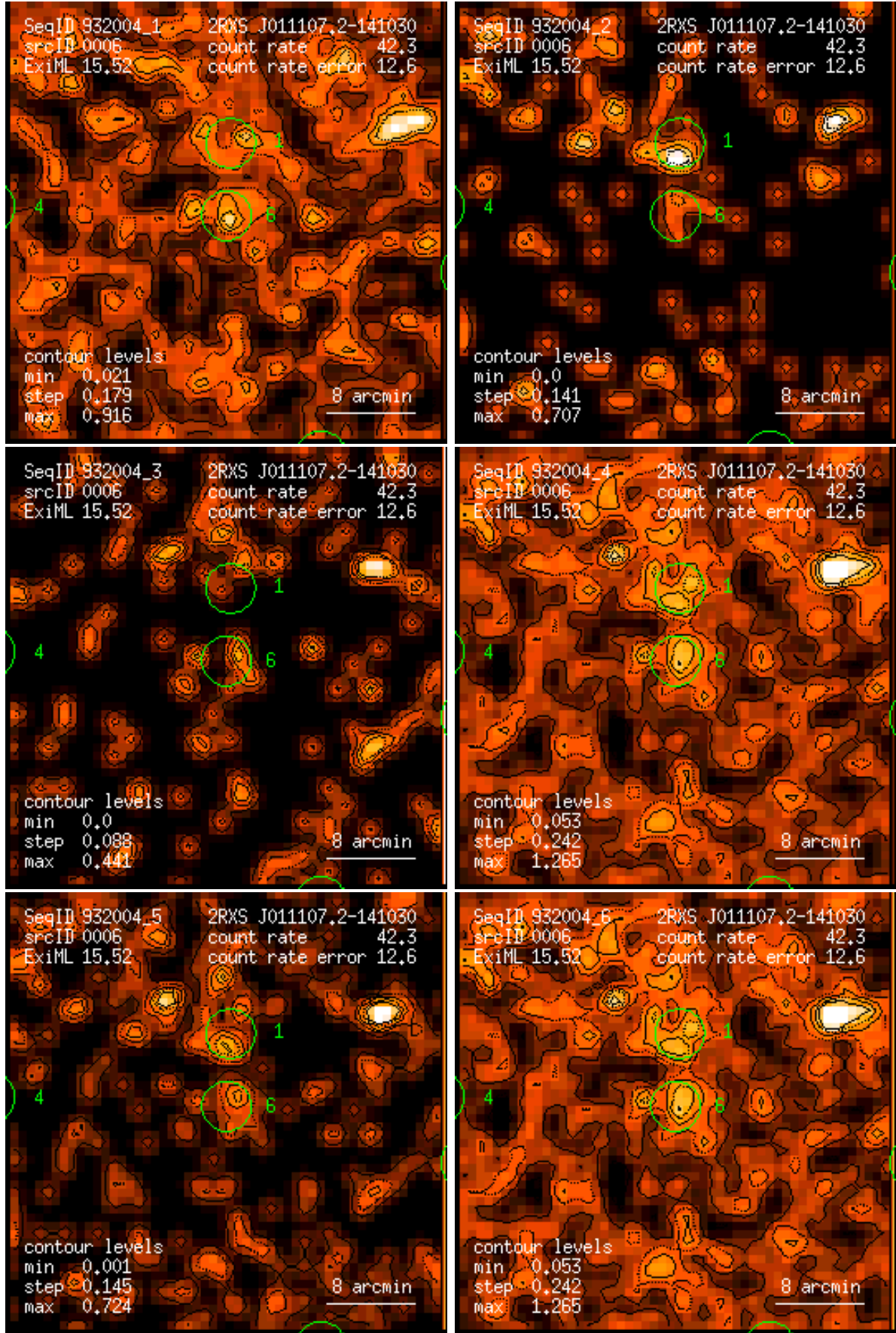
Figure 6: RASS 932004: detection 0006: band rate images, Gaussian filter: (1) PSPC channels 11 – 41, (2) 52 – 90, (3) 91 – 201, (4) 11 – 235, (5) 52 – 201, (6) 11 – 201. Broad band rates in counts/ks. Band rate contour levels in counts/ks/arcmin 2 .
