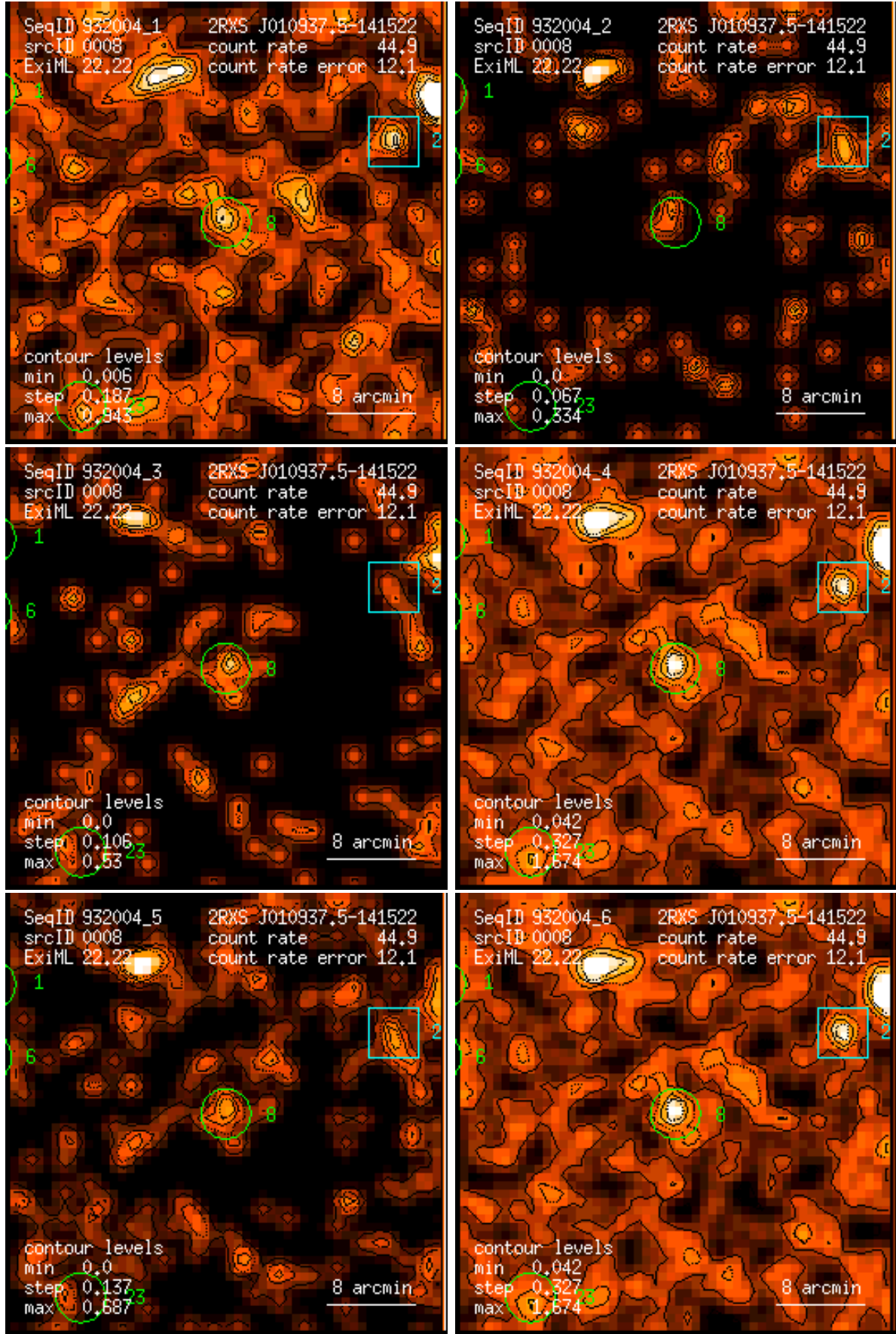
Figure 8: RASS 932004: detection 0008: band rate images, Gaussian filter: (1) PSPC channels 11 – 41, (2) 52 – 90, (3) 91 – 201, (4) 11 – 235, (5) 52 – 201, (6) 11 – 201. Broad band rates in counts/ks. Band rate contour levels in counts/ks/arcmin 2 .
