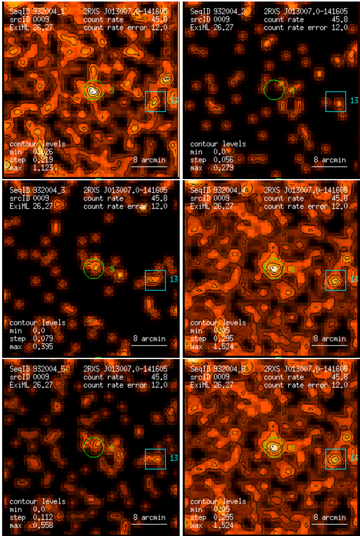
Figure 9: RASS 932004: detection 0009: band rate images, Gaussian filter: (1) PSPC channels 11 – 41, (2) 52 – 90, (3) 91 – 201, (4) 11 – 235, (5) 52 – 201, (6) 11 – 201. Broad band rates in counts/ks. Band rate contour levels in counts/ks/arcmin 2 .
