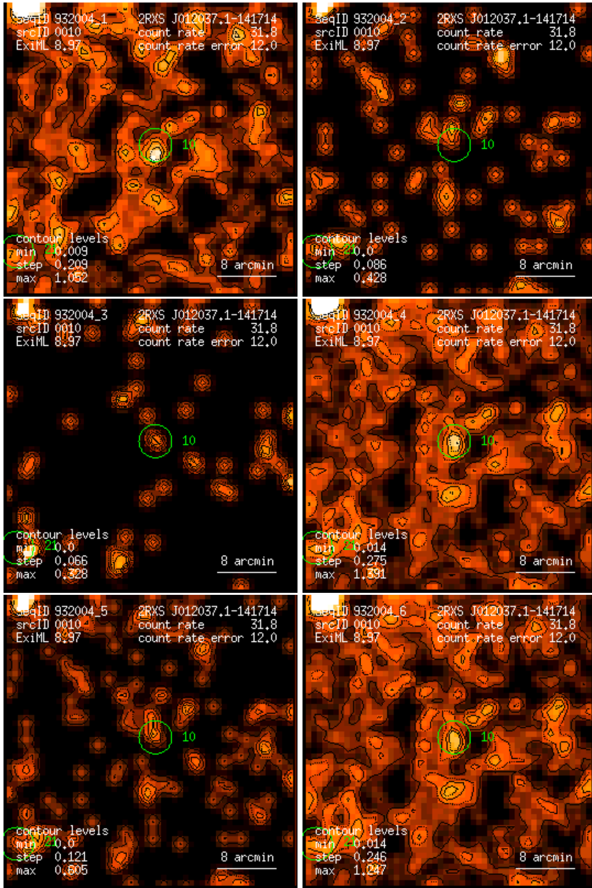
Figure 10: RASS 932004: detection 0010: band rate images, Gaussian filter: (1) PSPC channels 11 – 41, (2) 52 – 90, (3) 91 – 201, (4) 11 – 235, (5) 52 – 201, (6) 11 – 201. Broad band rates in counts/ks. Band rate contour levels in counts/ks/arcmin 2 .
