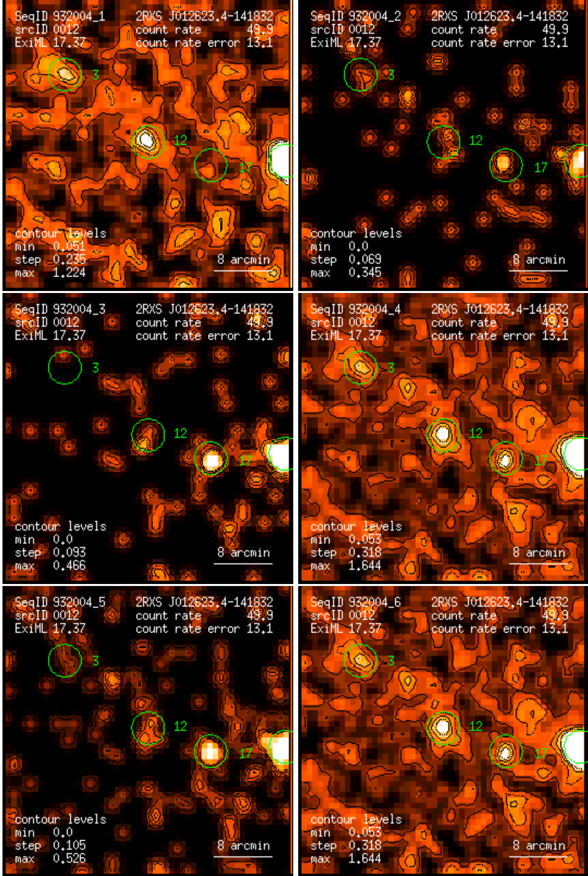
Figure 12: RASS 932004: detection 0012: band rate images, Gaussian filter: (1) PSPC channels 11 – 41, (2) 52 – 90, (3) 91 – 201, (4) 11 – 235, (5) 52 – 201, (6) 11 – 201. Broad band rates in counts/ks. Band rate contour levels in counts/ks/arcmin 2 .
