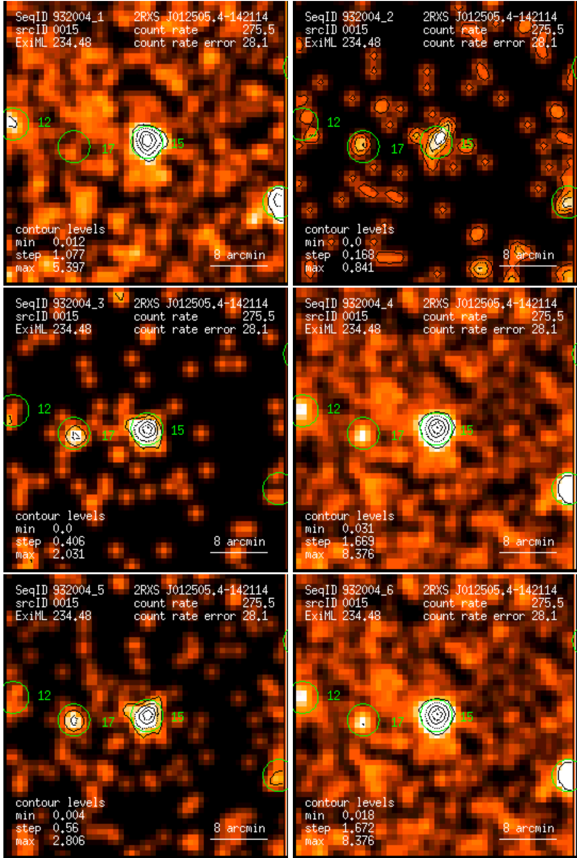
Figure 15: RASS 932004: detection 0015: band rate images, Gaussian filter: (1) PSPC channels 11 – 41, (2) 52 – 90, (3) 91 – 201, (4) 11 – 235, (5) 52 – 201, (6) 11 – 201. Broad band rates in counts/ks. Band rate contour levels in counts/ks/arcmin 2 .
