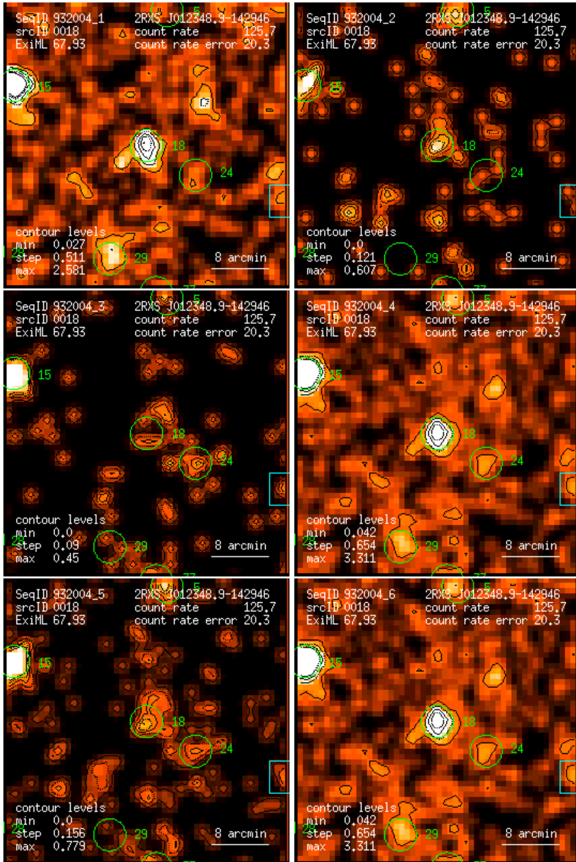
Figure 18: RASS 932004: detection 0018: band rate images, Gaussian filter: (1) PSPC channels 11 – 41, (2) 52 – 90, (3) 91 – 201, (4) 11 – 235, (5) 52 – 201, (6) 11 – 201. Broad band rates in counts/ks. Band rate contour levels in counts/ks/arcmin 2 .
