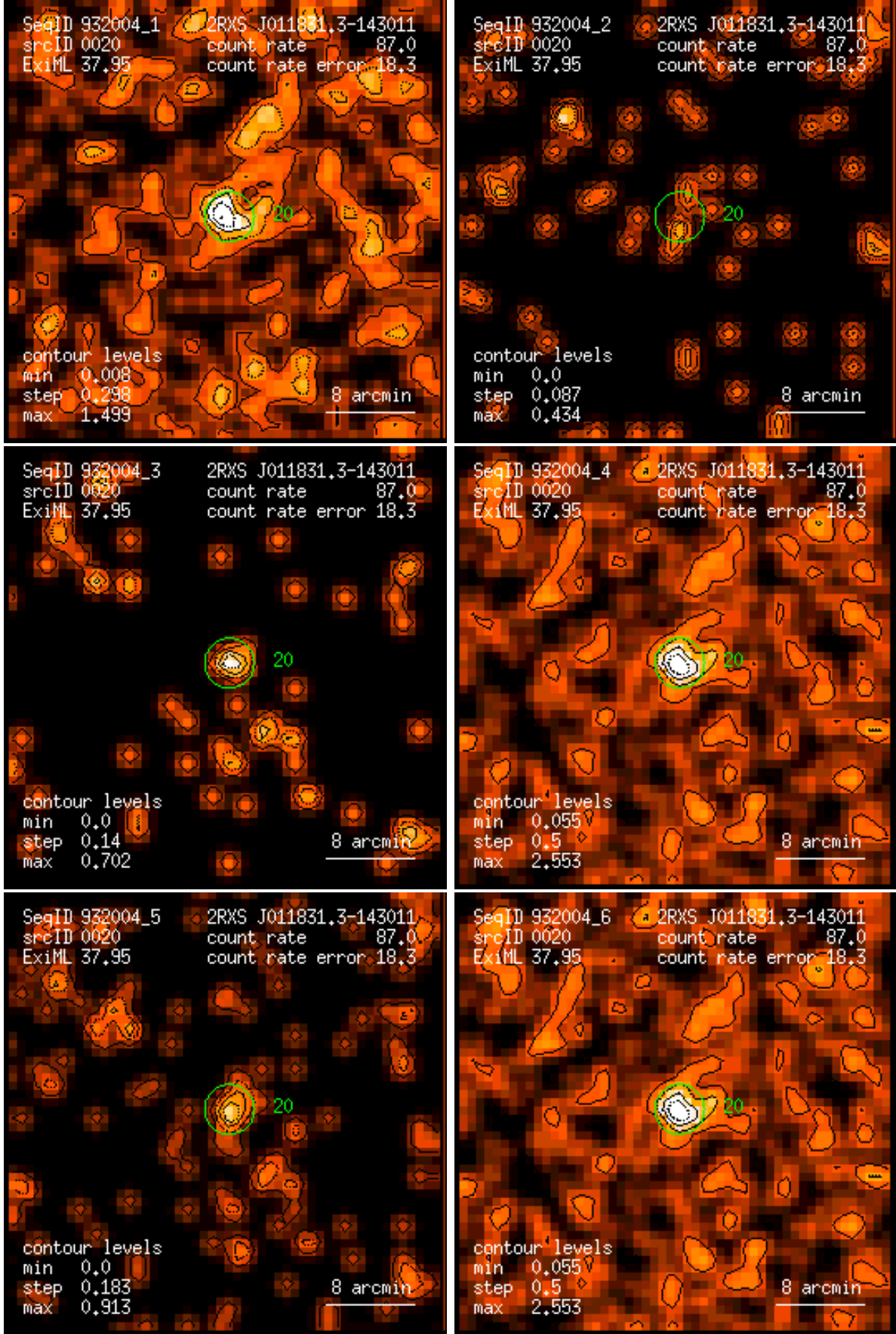
Figure 20: RASS 932004: detection 0020: band rate images, Gaussian filter: (1) PSPC channels 11 – 41, (2) 52 – 90, (3) 91 – 201, (4) 11 – 235, (5) 52 – 201, (6) 11 – 201. Broad band rates in counts/ks. Band rate contour levels in counts/ks/arcmin 2 .
