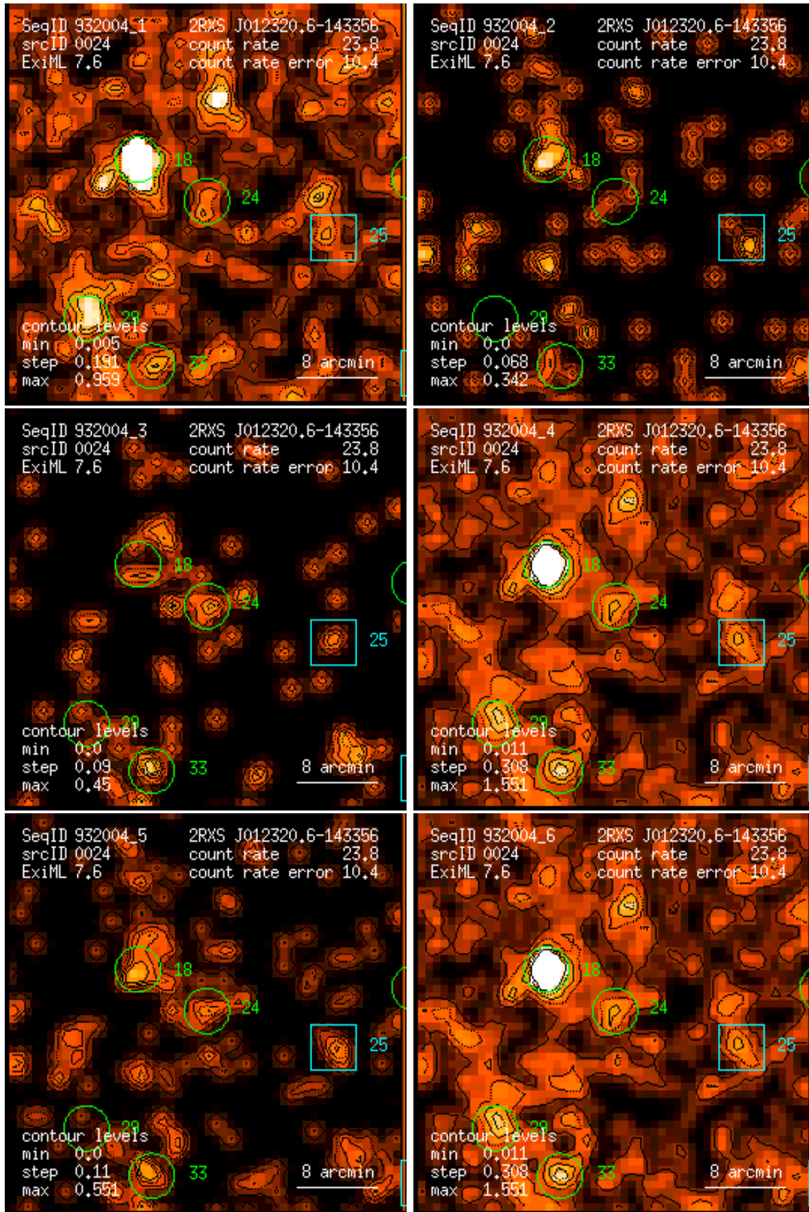
Figure 24: RASS 932004: detection 0024: band rate images, Gaussian filter: (1) PSPC channels 11 – 41, (2) 52 – 90, (3) 91 – 201, (4) 11 – 235, (5) 52 – 201, (6) 11 – 201. Broad band rates in counts/ks. Band rate contour levels in counts/ks/arcmin 2 .
