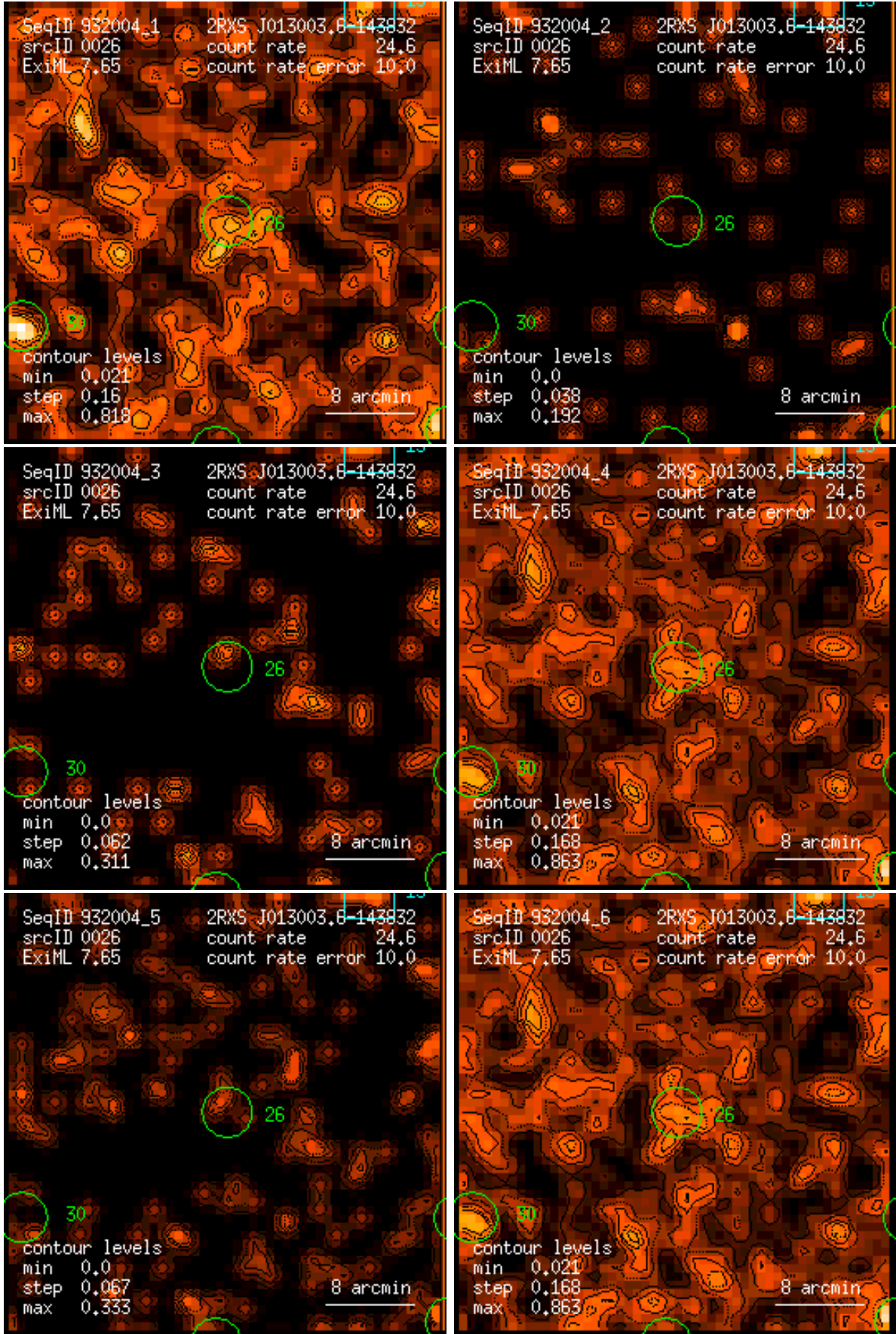
Figure 26: RASS 932004: detection 0026: band rate images, Gaussian filter: (1) PSPC channels 11 – 41, (2) 52 – 90, (3) 91 – 201, (4) 11 – 235, (5) 52 – 201, (6) 11 – 201. Broad band rates in counts/ks. Band rate contour levels in counts/ks/arcmin 2 .
