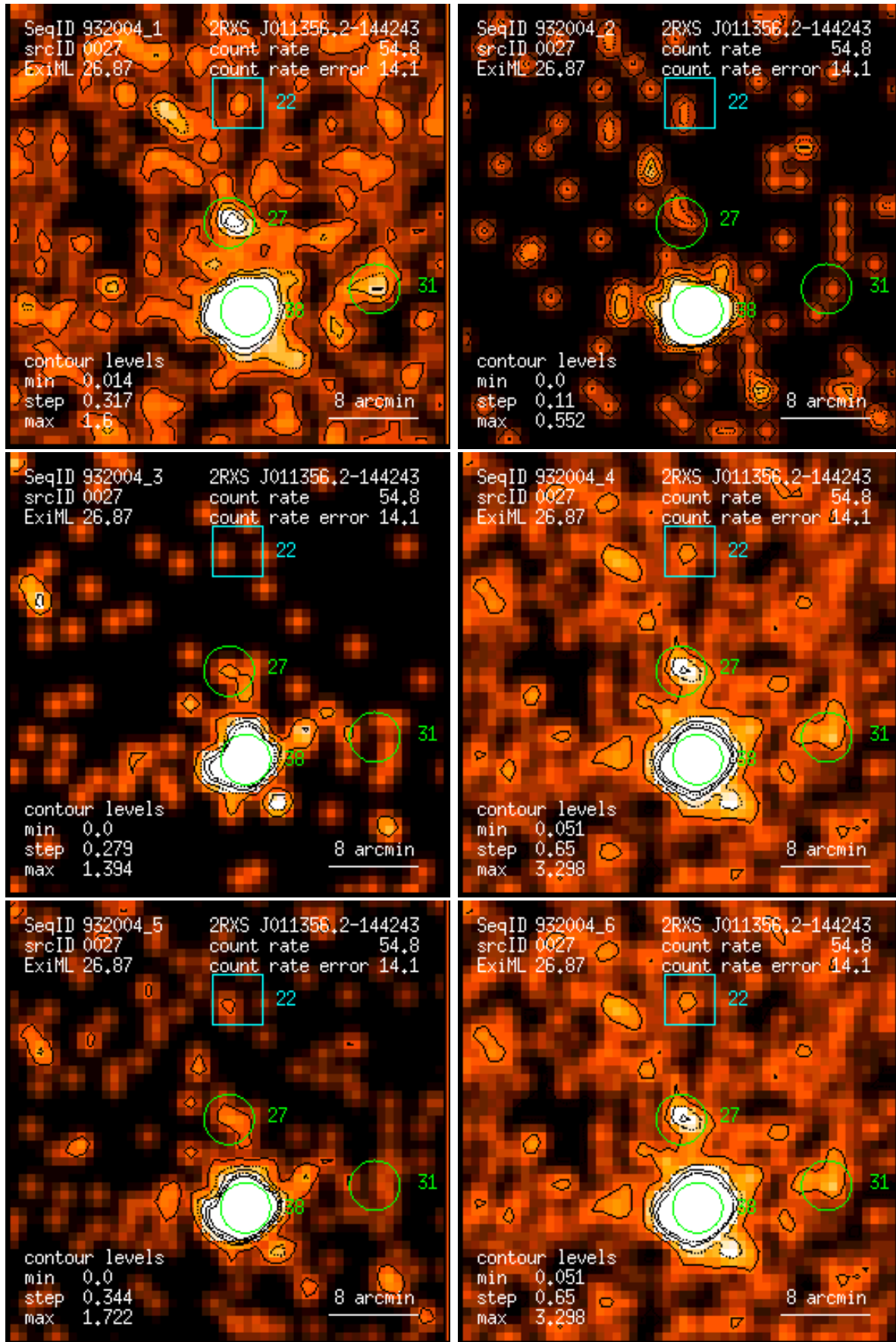
Figure 27: RASS 932004: detection 0027: band rate images, Gaussian filter: (1) PSPC channels 11 – 41, (2) 52 – 90, (3) 91 – 201, (4) 11 – 235, (5) 52 – 201, (6) 11 – 201. Broad band rates in counts/ks. Band rate contour levels in counts/ks/arcmin 2 .
