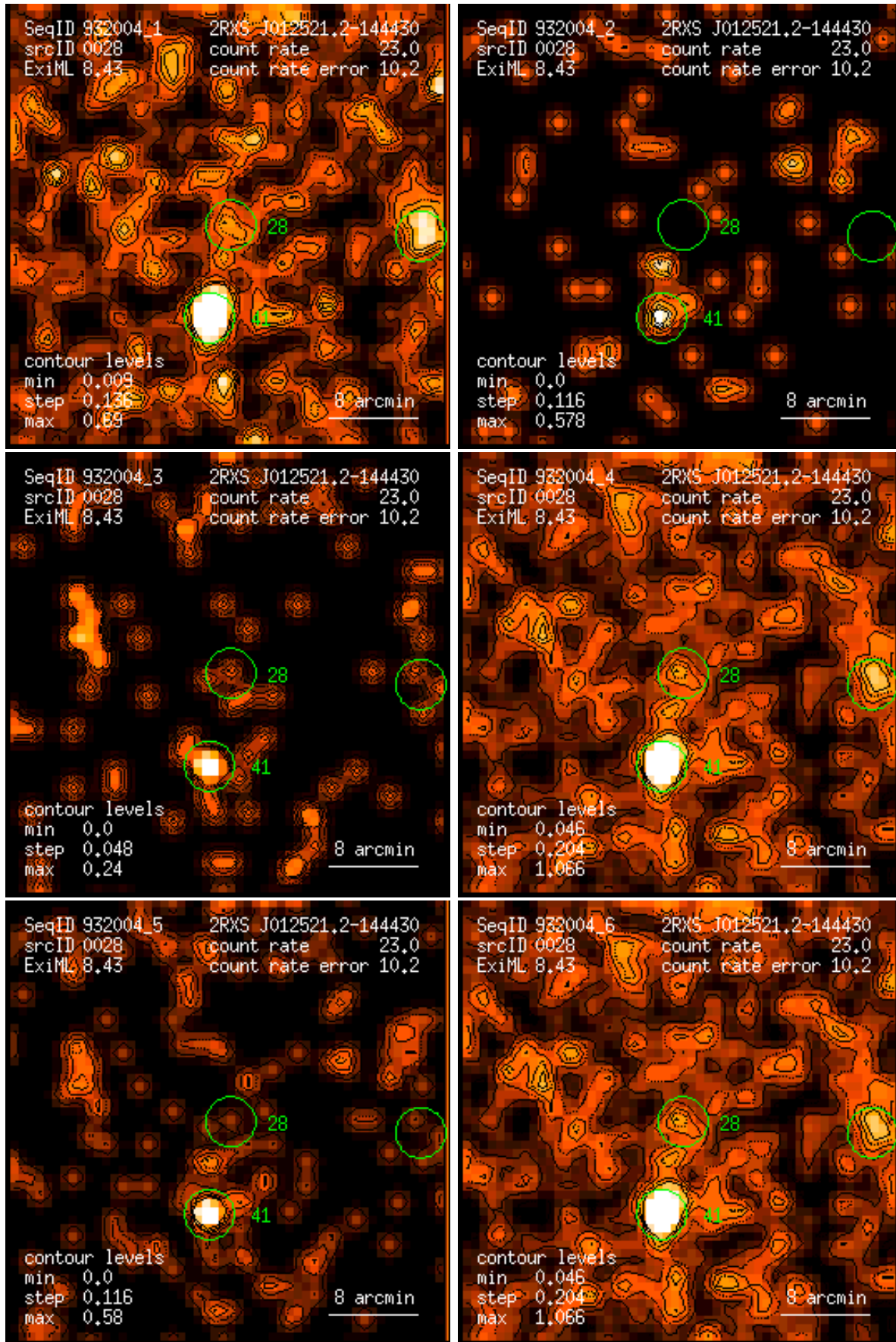
Figure 28: RASS 932004: detection 0028: band rate images, Gaussian filter: (1) PSPC channels 11 – 41, (2) 52 – 90, (3) 91 – 201, (4) 11 – 235, (5) 52 – 201, (6) 11 – 201. Broad band rates in counts/ks. Band rate contour levels in counts/ks/arcmin 2 .
