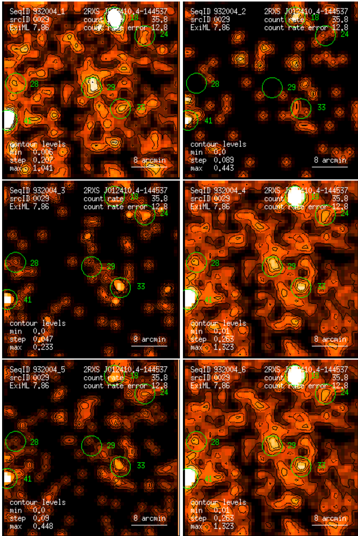
Figure 29: RASS 932004: detection 0029: band rate images, Gaussian filter: (1) PSPC channels 11 – 41, (2) 52 – 90, (3) 91 – 201, (4) 11 – 235, (5) 52 – 201, (6) 11 – 201. Broad band rates in counts/ks. Band rate contour levels in counts/ks/arcmin 2 .
