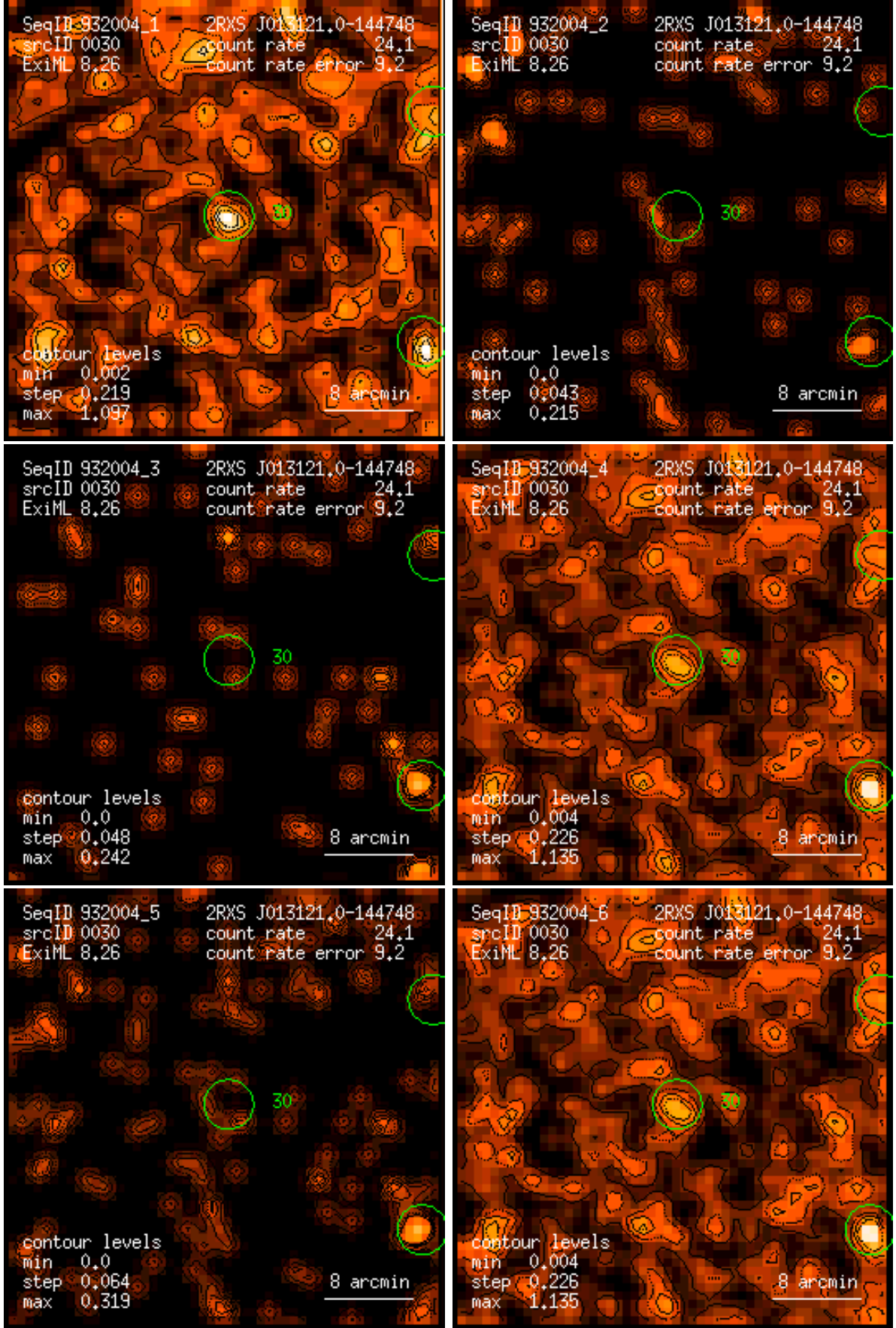
Figure 30: RASS 932004: detection 0030: band rate images, Gaussian filter: (1) PSPC channels 11 – 41, (2) 52 – 90, (3) 91 – 201, (4) 11 – 235, (5) 52 – 201, (6) 11 – 201. Broad band rates in counts/ks. Band rate contour levels in counts/ks/arcmin 2 .
