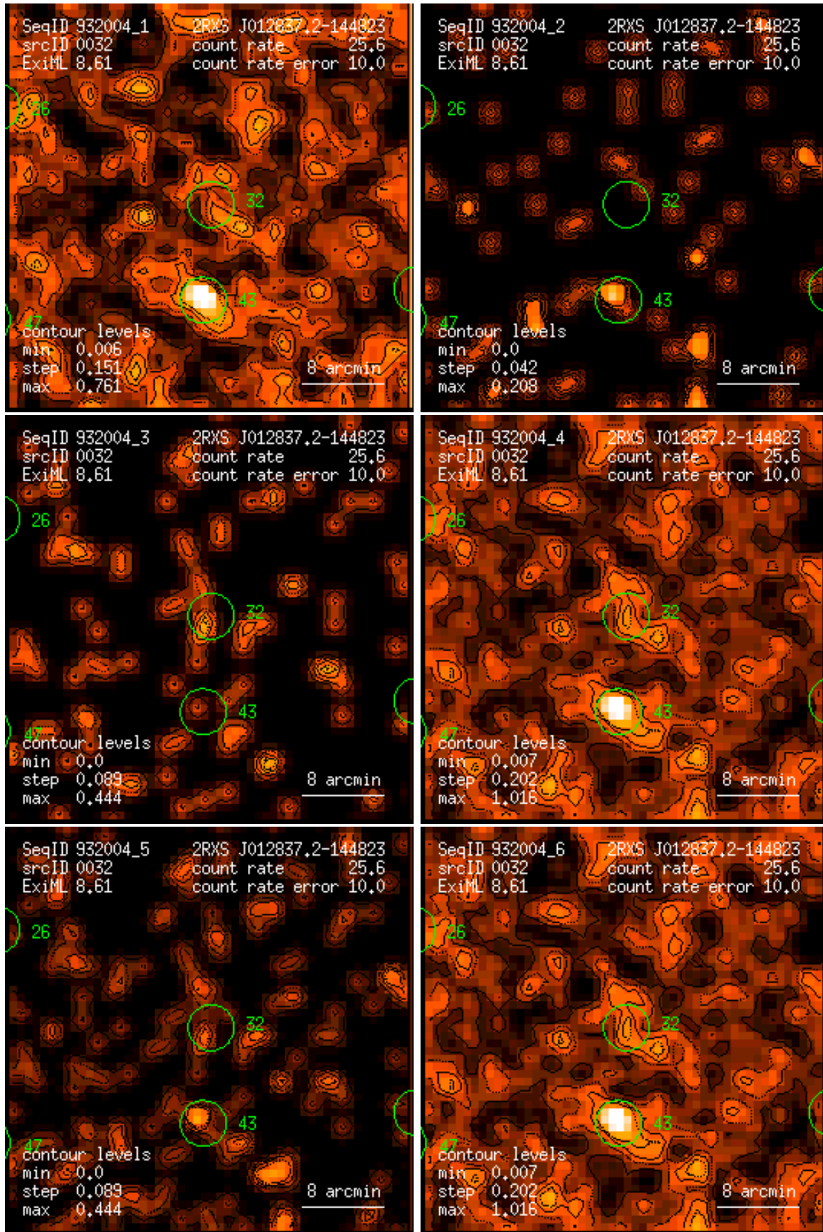
Figure 32: RASS 932004: detection 0032: band rate images, Gaussian filter: (1) PSPC channels 11 – 41, (2) 52 – 90, (3) 91 – 201, (4) 11 – 235, (5) 52 – 201, (6) 11 – 201. Broad band rates in counts/ks. Band rate contour levels in counts/ks/arcmin 2 .
