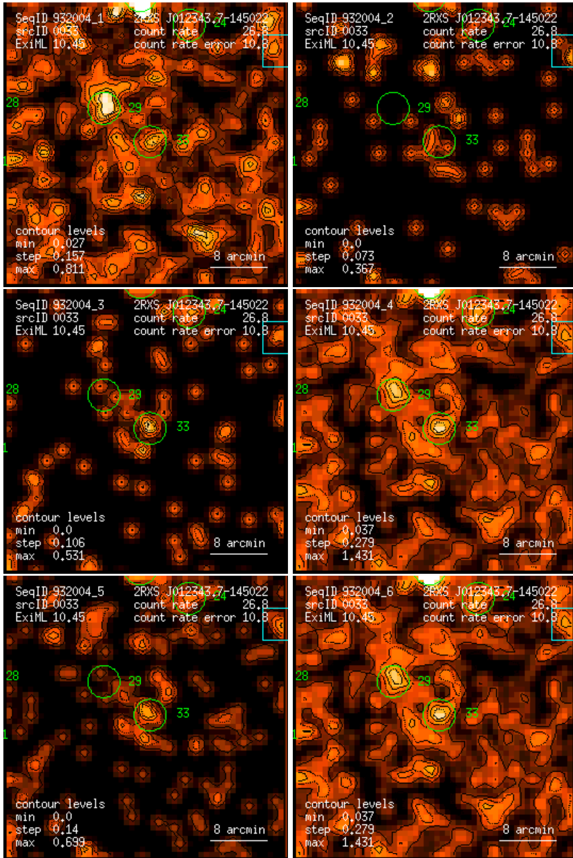
Figure 33: RASS 932004: detection 0033: band rate images, Gaussian filter: (1) PSPC channels 11 – 41, (2) 52 – 90, (3) 91 – 201, (4) 11 – 235, (5) 52 – 201, (6) 11 – 201. Broad band rates in counts/ks. Band rate contour levels in counts/ks/arcmin 2 .
