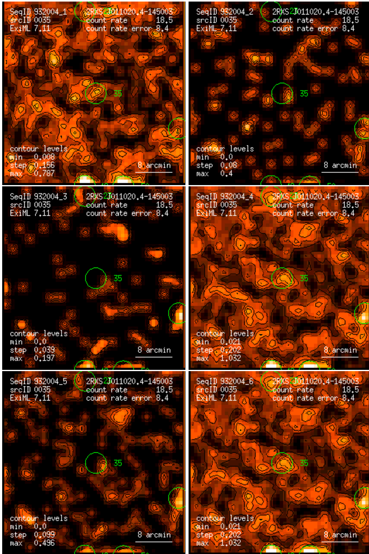
Figure 35: RASS 932004: detection 0035: band rate images, Gaussian filter: (1) PSPC channels 11 – 41, (2) 52 – 90, (3) 91 – 201, (4) 11 – 235, (5) 52 – 201, (6) 11 – 201. Broad band rates in counts/ks. Band rate contour levels in counts/ks/arcmin 2 .
