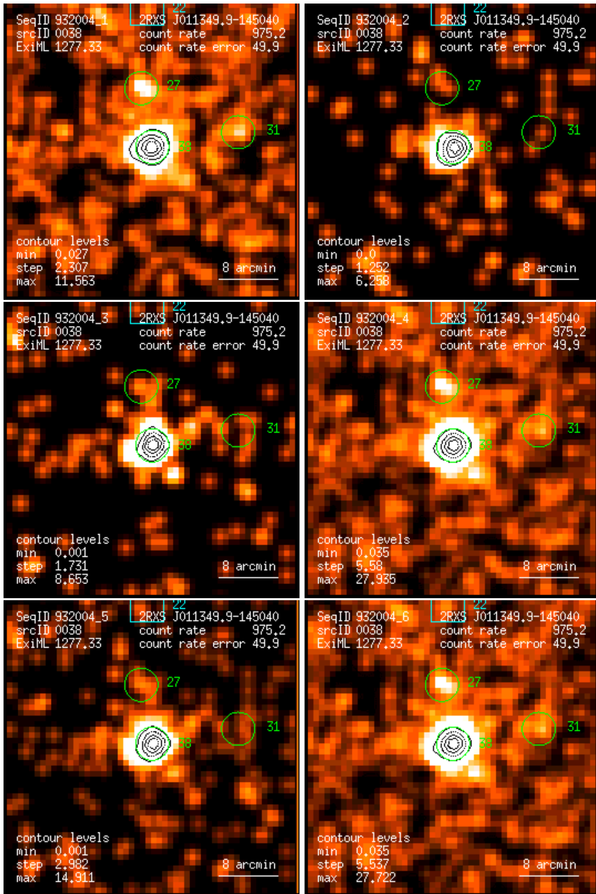
Figure 38: RASS 932004: detection 0038: band rate images, Gaussian filter: (1) PSPC channels 11 – 41, (2) 52 – 90, (3) 91 – 201, (4) 11 – 235, (5) 52 – 201, (6) 11 – 201. Broad band rates in counts/ks. Band rate contour levels in counts/ks/arcmin 2 .
