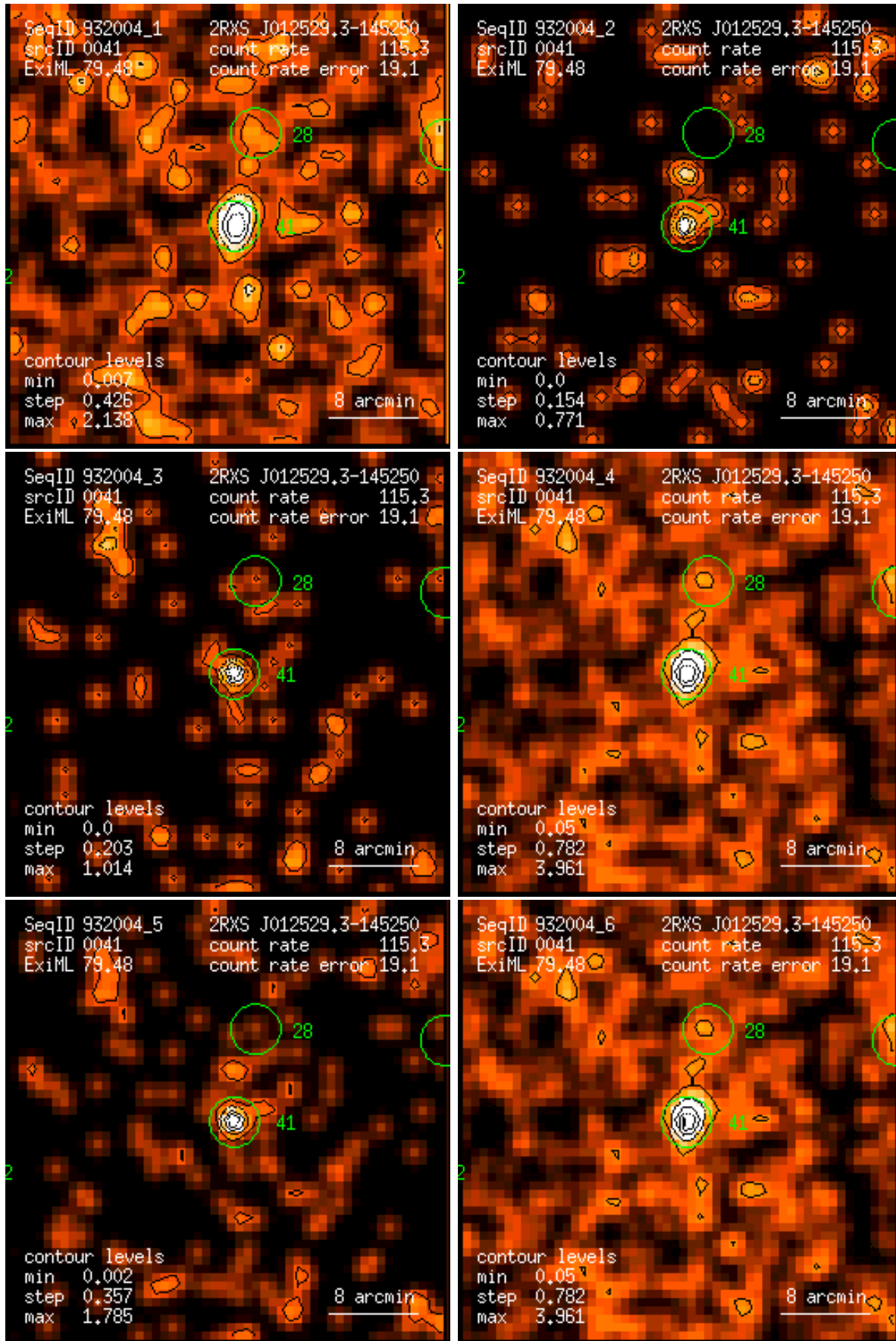
Figure 41: RASS 932004: detection 0041: band rate images, Gaussian filter: (1) PSPC channels 11 – 41, (2) 52 – 90, (3) 91 – 201, (4) 11 – 235, (5) 52 – 201, (6) 11 – 201. Broad band rates in counts/ks. Band rate contour levels in counts/ks/arcmin 2 .
