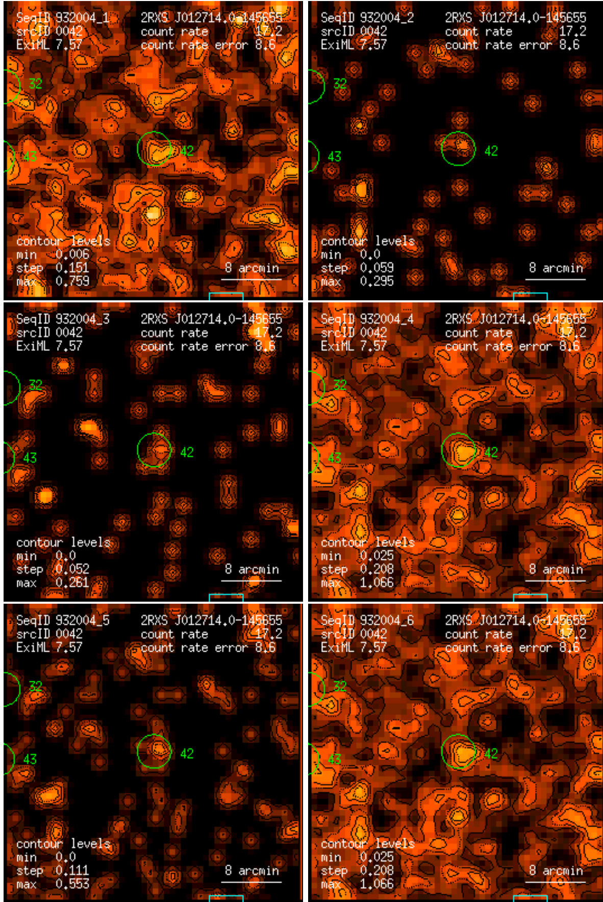
Figure 42: RASS 932004: detection 0042: band rate images, Gaussian filter: (1) PSPC channels 11 – 41, (2) 52 – 90, (3) 91 – 201, (4) 11 – 235, (5) 52 – 201, (6) 11 – 201. Broad band rates in counts/ks. Band rate contour levels in counts/ks/arcmin 2 .
