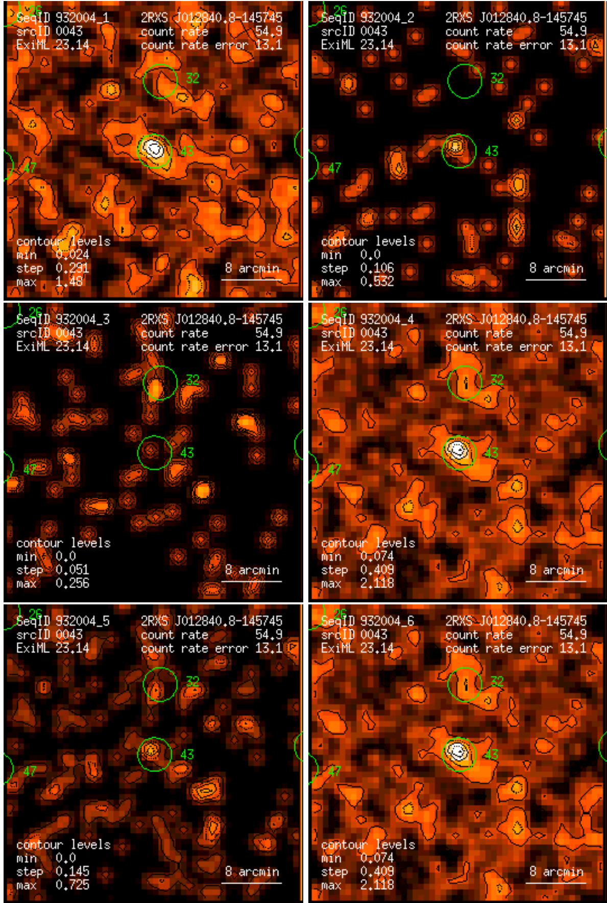
Figure 43: RASS 932004: detection 0043: band rate images, Gaussian filter: (1) PSPC channels 11 – 41, (2) 52 – 90, (3) 91 – 201, (4) 11 – 235, (5) 52 – 201, (6) 11 – 201. Broad band rates in counts/ks. Band rate contour levels in counts/ks/arcmin 2 .
