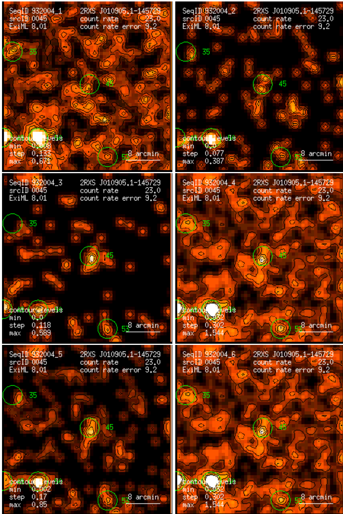
Figure 45: RASS 932004: detection 0045: band rate images, Gaussian filter: (1) PSPC channels 11 – 41, (2) 52 – 90, (3) 91 – 201, (4) 11 – 235, (5) 52 – 201, (6) 11 – 201. Broad band rates in counts/ks. Band rate contour levels in counts/ks/arcmin 2 .
