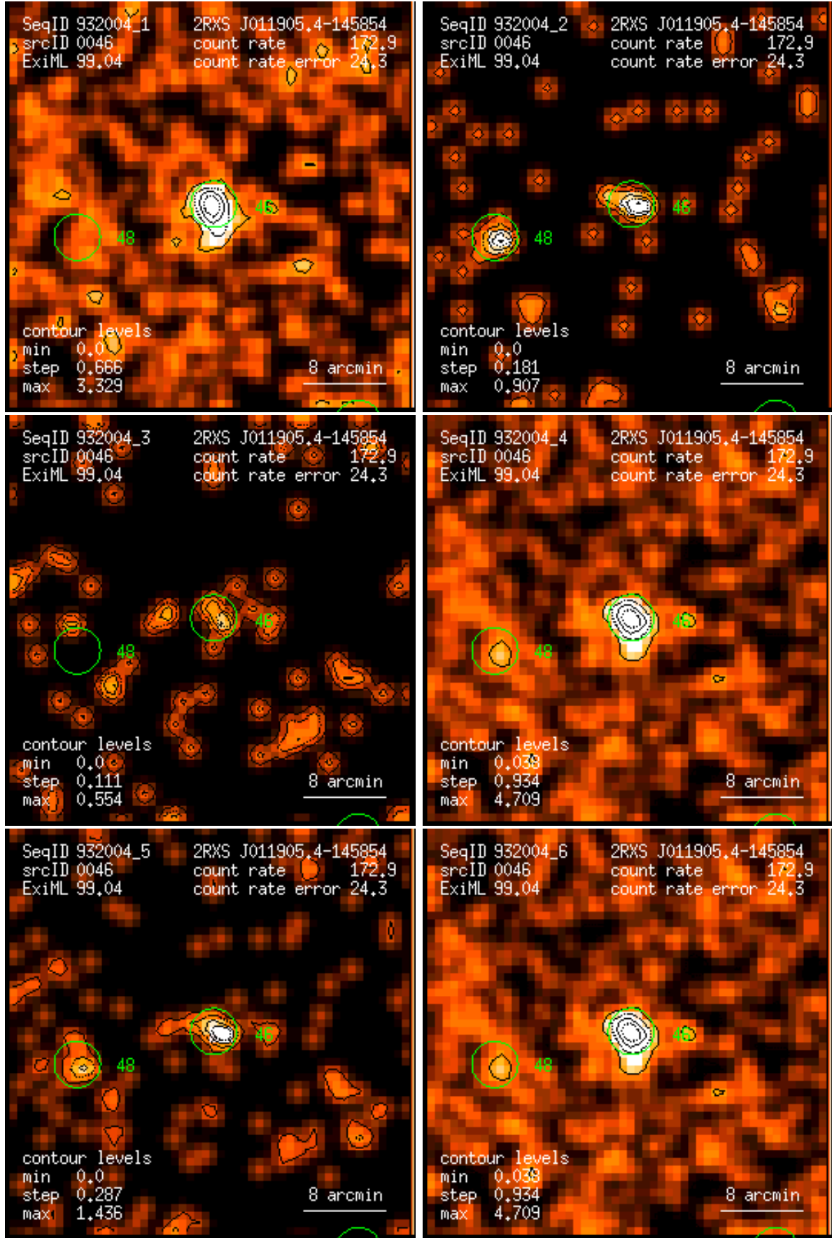
Figure 46: RASS 932004: detection 0046: band rate images, Gaussian filter: (1) PSPC channels 11 – 41, (2) 52 – 90, (3) 91 – 201, (4) 11 – 235, (5) 52 – 201, (6) 11 – 201. Broad band rates in counts/ks. Band rate contour levels in counts/ks/arcmin 2 .
