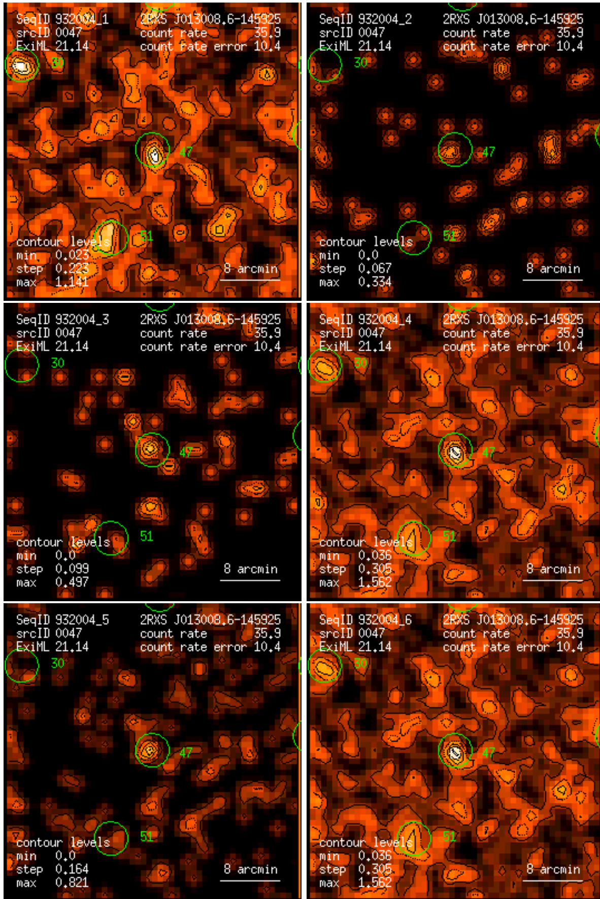
Figure 47: RASS 932004: detection 0047: band rate images, Gaussian filter: (1) PSPC channels 11 – 41, (2) 52 – 90, (3) 91 – 201, (4) 11 – 235, (5) 52 – 201, (6) 11 – 201. Broad band rates in counts/ks. Band rate contour levels in counts/ks/arcmin 2 .
