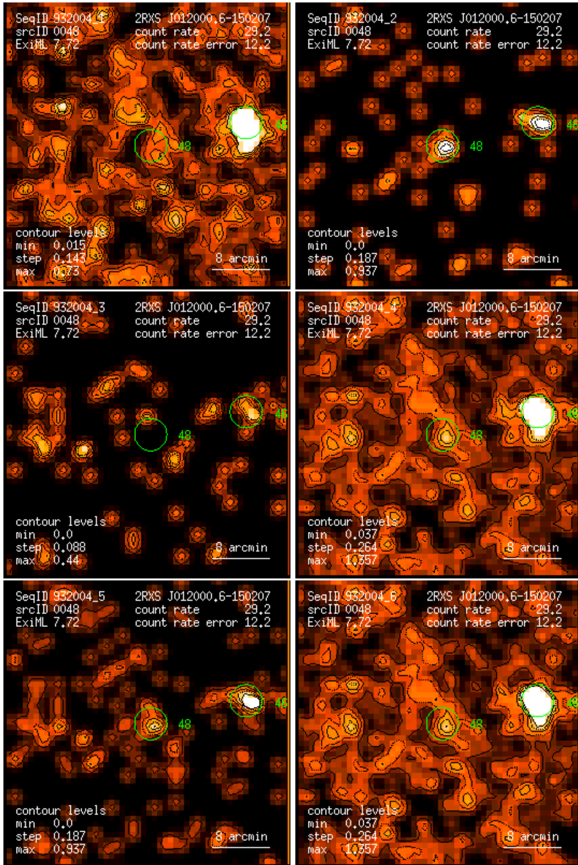
Figure 48: RASS 932004: detection 0048: band rate images, Gaussian filter: (1) PSPC channels 11 – 41, (2) 52 – 90, (3) 91 – 201, (4) 11 – 235, (5) 52 – 201, (6) 11 – 201. Broad band rates in counts/ks. Band rate contour levels in counts/ks/arcmin 2 .
