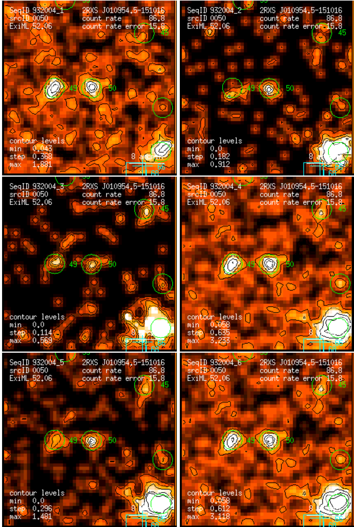
Figure 50: RASS 932004: detection 0050: band rate images, Gaussian filter: (1) PSPC channels 11 – 41, (2) 52 – 90, (3) 91 – 201, (4) 11 – 235, (5) 52 – 201, (6) 11 – 201. Broad band rates in counts/ks. Band rate contour levels in counts/ks/arcmin 2 .
